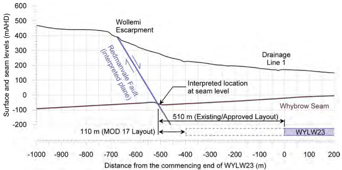
Fig. 1.6 Section through the Redmanvale Fault and the commencing end of WYLW23
