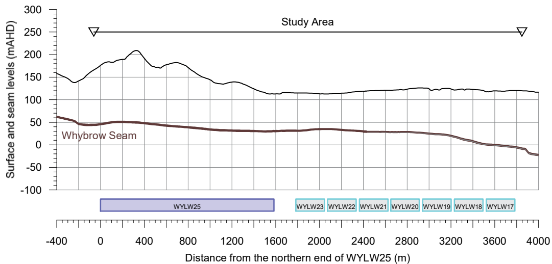
Fig. 1.2 Surface and seam levels along Section 1 through WYLW17 to WYLW23 and the centreline of WYLW25
