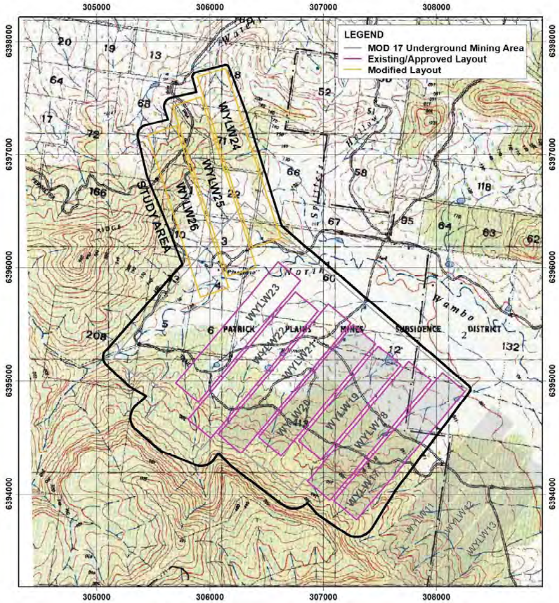
Fig. 2.1 WYLNW17 to WYLNW26 overlaid on CMA Map No. Doyles Creek 9032-1-N
