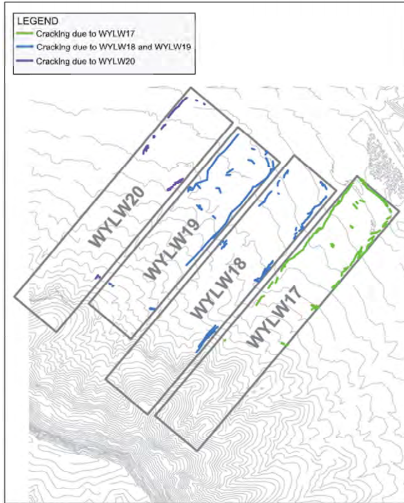
Fig. 4.3 Mapped surface cracking above WYLR17 to WYLR21
