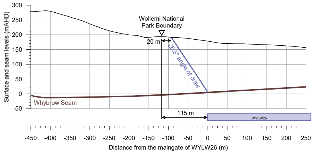
Fig. 5.30 Section through the Wollemi National Park and the modified WYLR26
