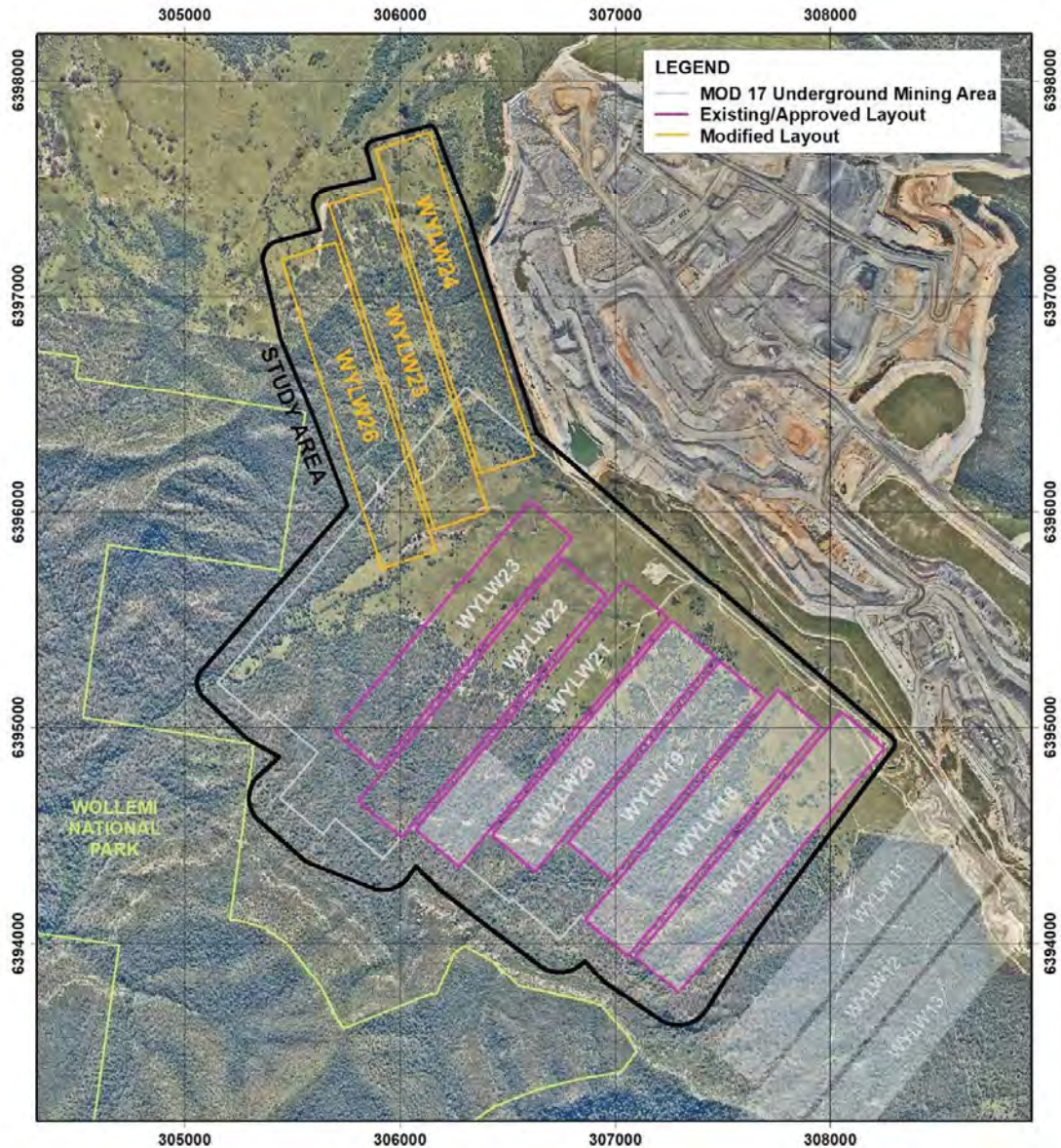
Fig. 5.32 WYLW17 to WYLW26 and the Study Area
