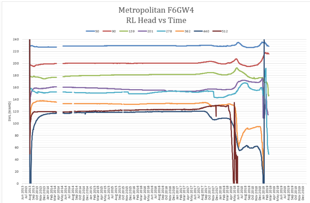
Figure 5.6 Piezometer levels over the period 2013 to early 2019 at borehole F6GW4 (source: HydroSimulations, 2019)
