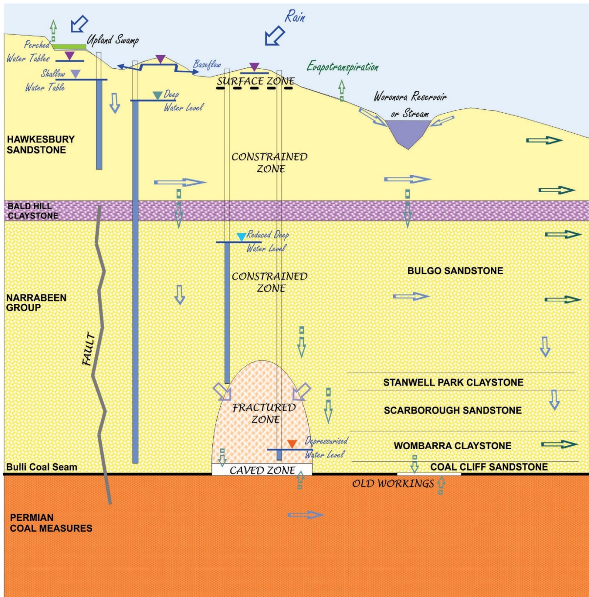
Figure 2.1. Conceptual groundwater system for Metropolitan Coal mining conditions (not to scale)
