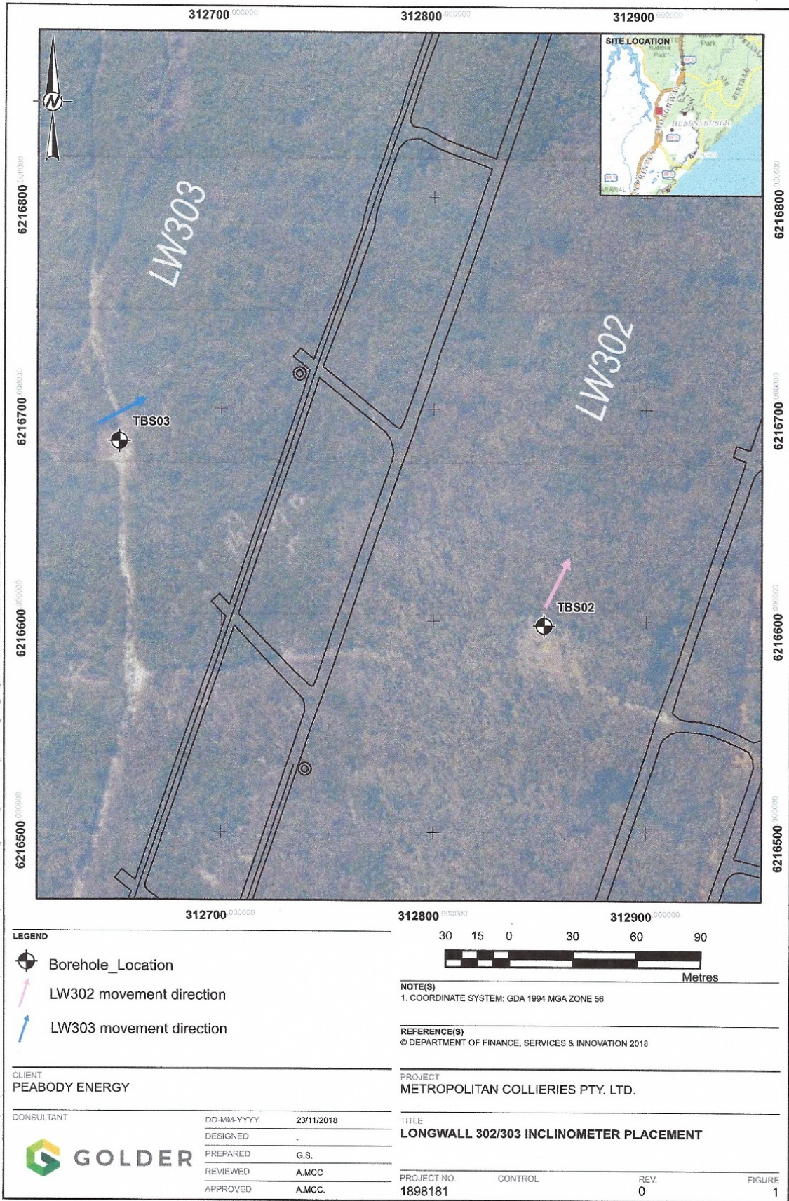
Figure 4.2 Location of borehole inclinometers TBS02 and TBS03 (source: Golder Longwall 302 TBS02, TBS03 Results)
