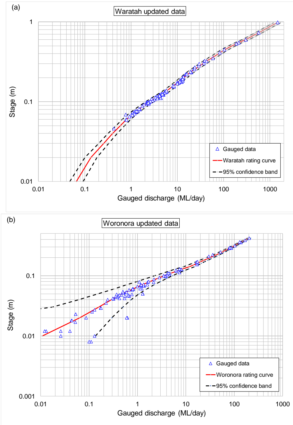
Figure A2. Rating curve for (a) Waratah Rivulet (GS2132102) and (b) Woronora River (GS2132101) showing the 95% uncertainty band
