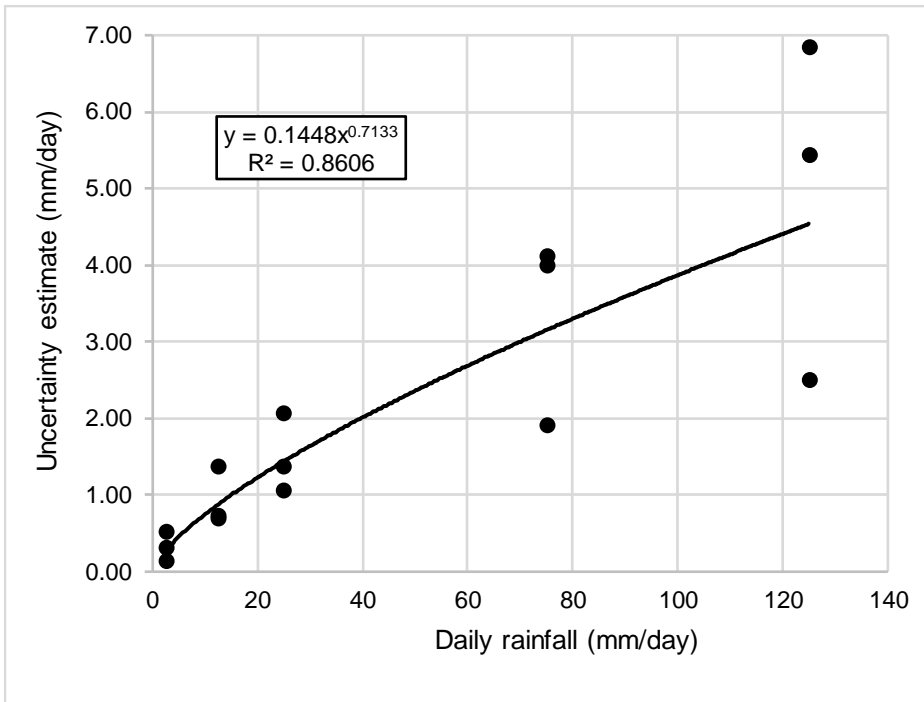
Figure A1. Uncertainty estimates (standard error) based on daily rainfall estimates from Table A2
