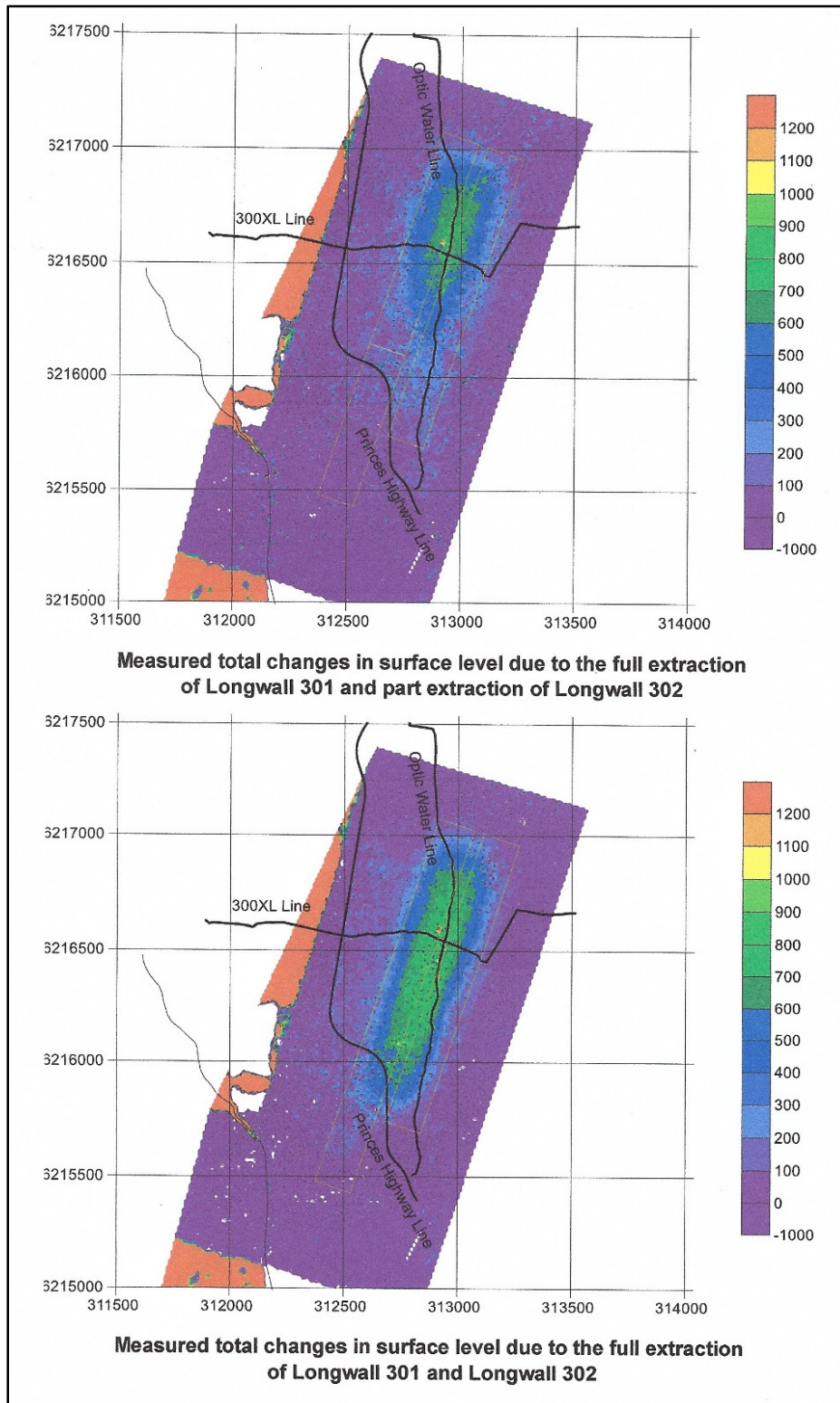
Figure 4.12 LIDAR survey results after LW301 and LW302 (source: MSEC)
