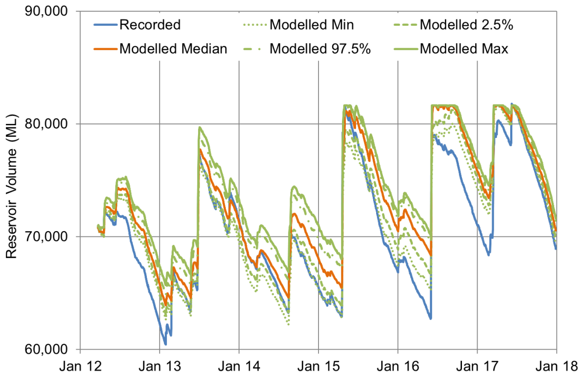
Figure 10 Woronora Reservoir Volume Uncertainty
