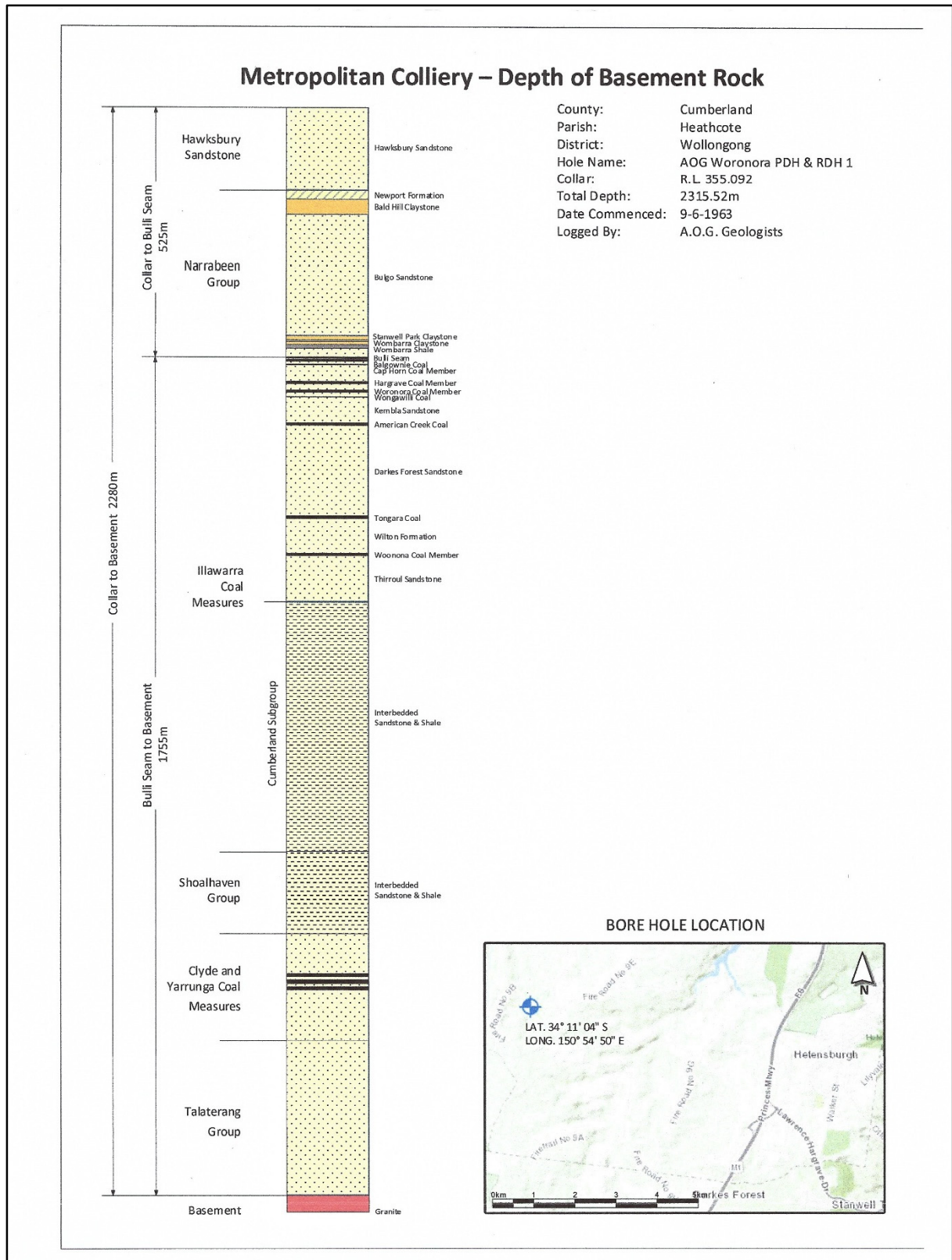
Figure 4.7 Surface to basement geological section – Metropolitan Coal (source: Metropolitan Coal)
