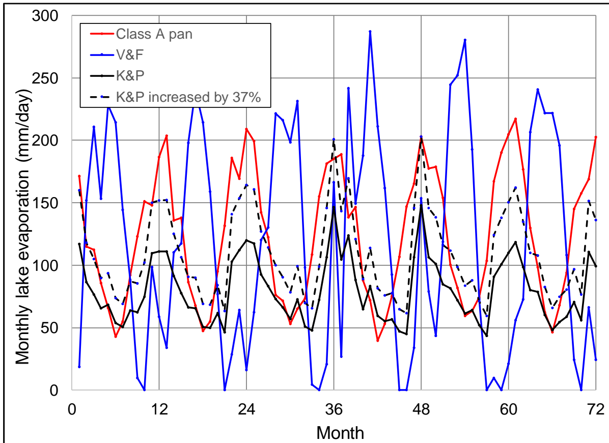
Figure 6.7 Estimates of monthly lake evaporation (V&F: Vardavas and Fountoulakis (1996) and K&P: Kohler and Parmele (1967)) compared with Class A pan SILO DD estimates for Woronora Reservoir
