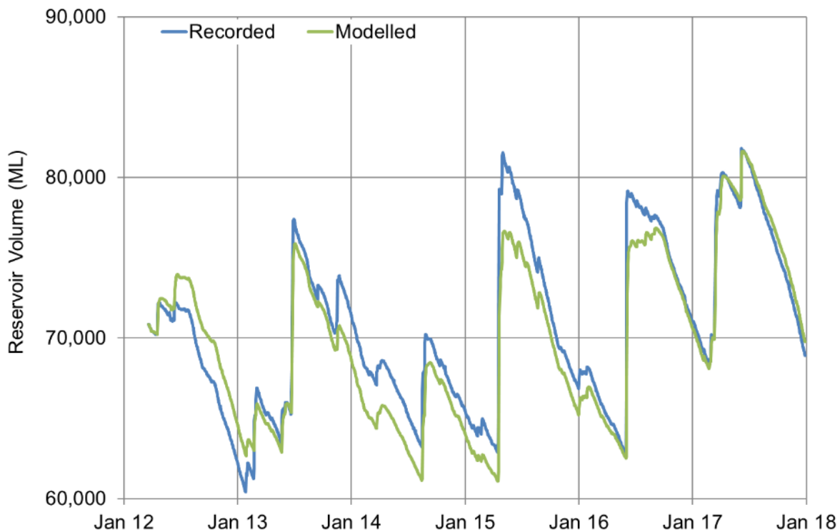
Figure 8 Comparison of Simulation Reservoir Volume and Recorded Reservoir Volume
