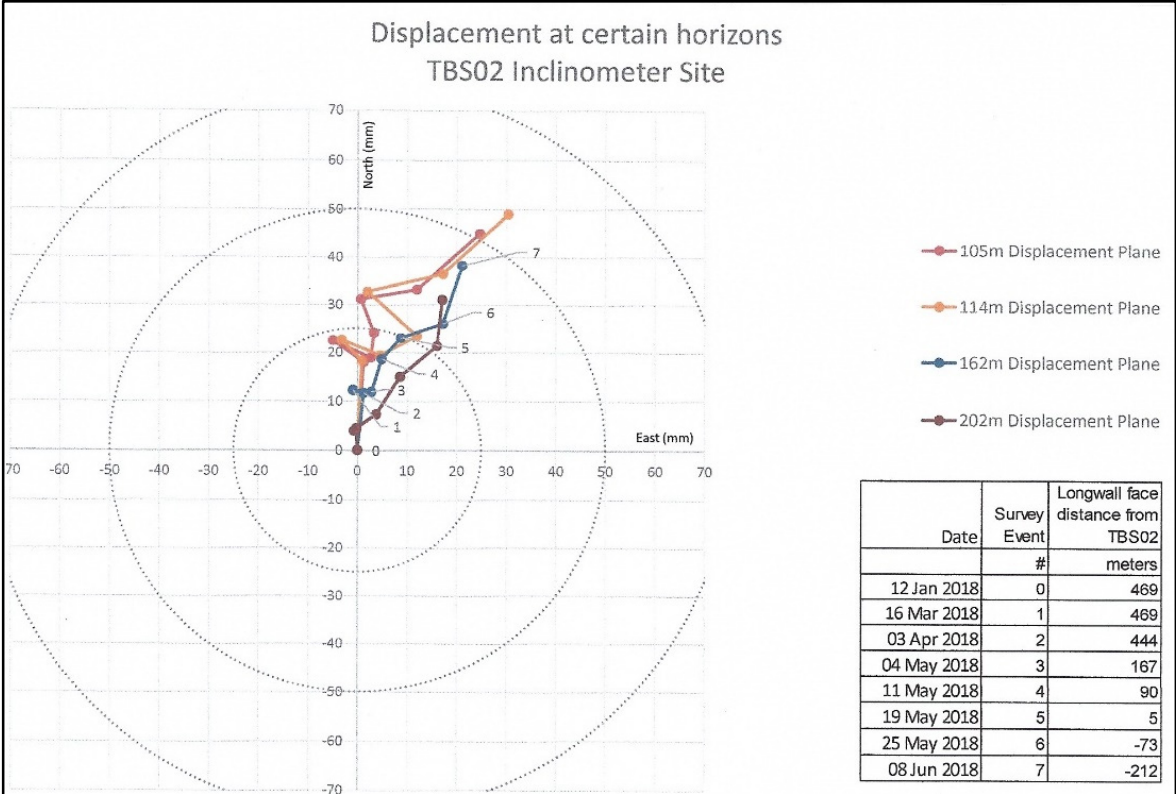
Figure 4.4 Inclinometer TBS02 – direction of movement for selected bedding plane horizons (source: Golder Longwall 302 TBS02, TBS03 Reports)
