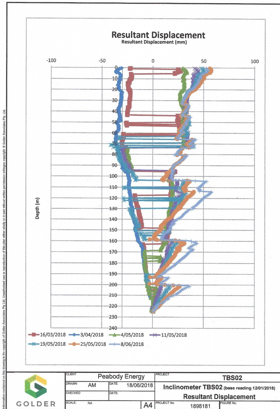
Figure 4.3 Borehole inclinometer TBS02 results (source: Golder Longwall 302 TBS02, TBS03 Results)
