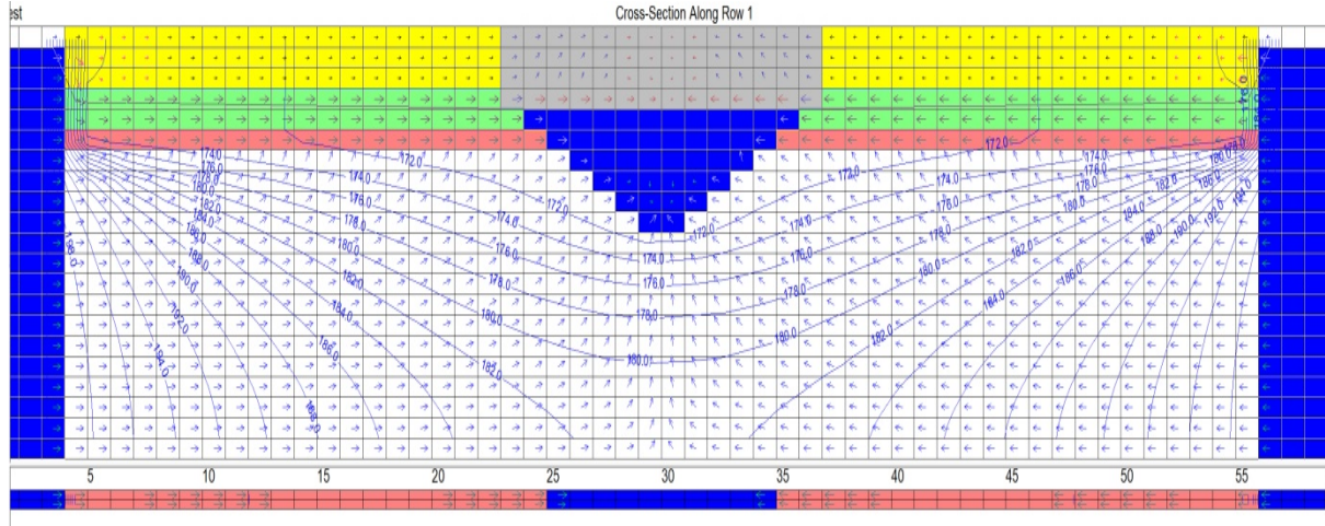
Figure E1. 2D 10 m thick idealised layered section with variable saturation MODFLOW numerical model with variable hydraulic conductivity with depth and Woronora Reservoir indicating flow vectors and hydraulic head contours.
