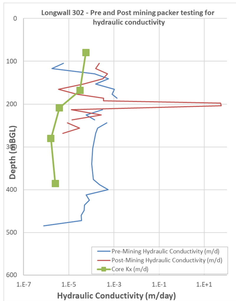
Figure 4.6 LW302 overburden conductivity test results – pre- and post-mining (source: HydroSimulations presentation – February 2019)
