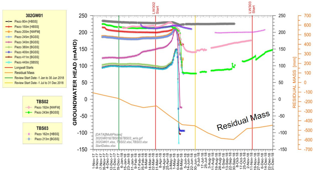
Figure 5.3 Pressure head graphs prior to, during and post longwall mining 302GW01
