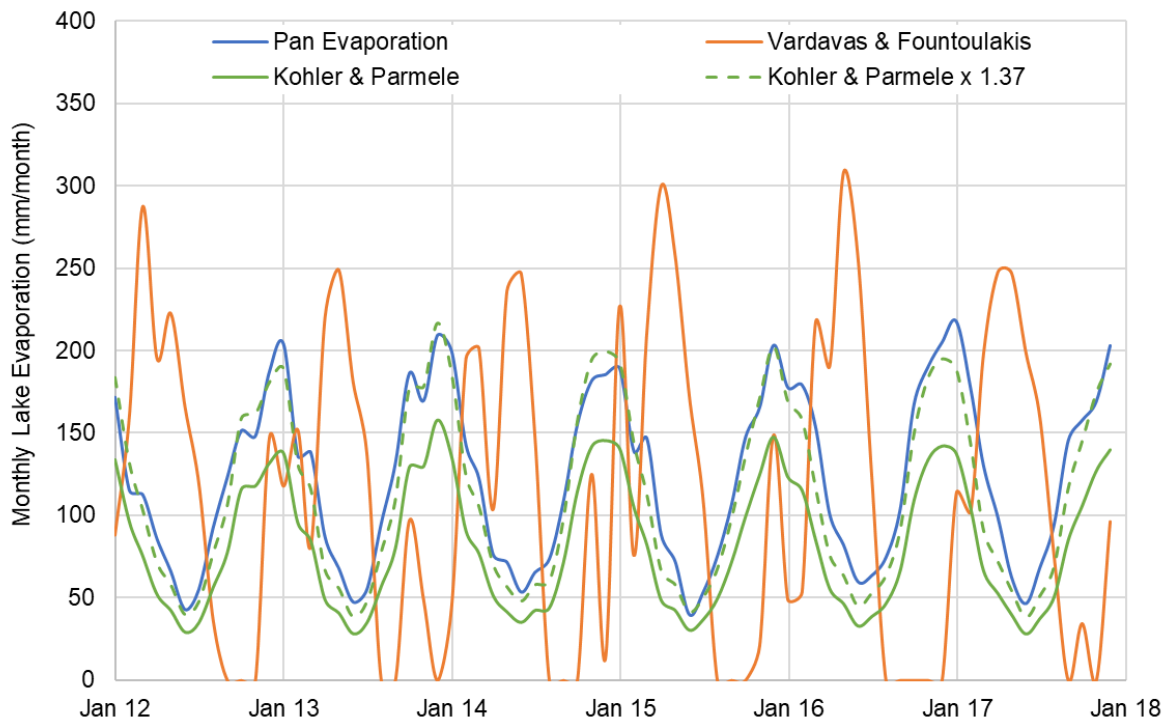
Figure 5 Comparison of Evaporation Rates
