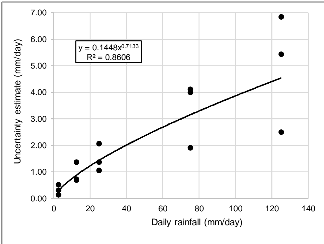
Figure F1. Uncertainty estimates (standard error) based on daily rainfall estimates from Table F2
