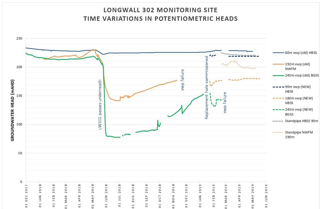
Figure 5.4 Extended piezometer pressure heads recovery in older 2018 and newer VWP's in 2019 (source: Metropolitan Coal, 2019)
