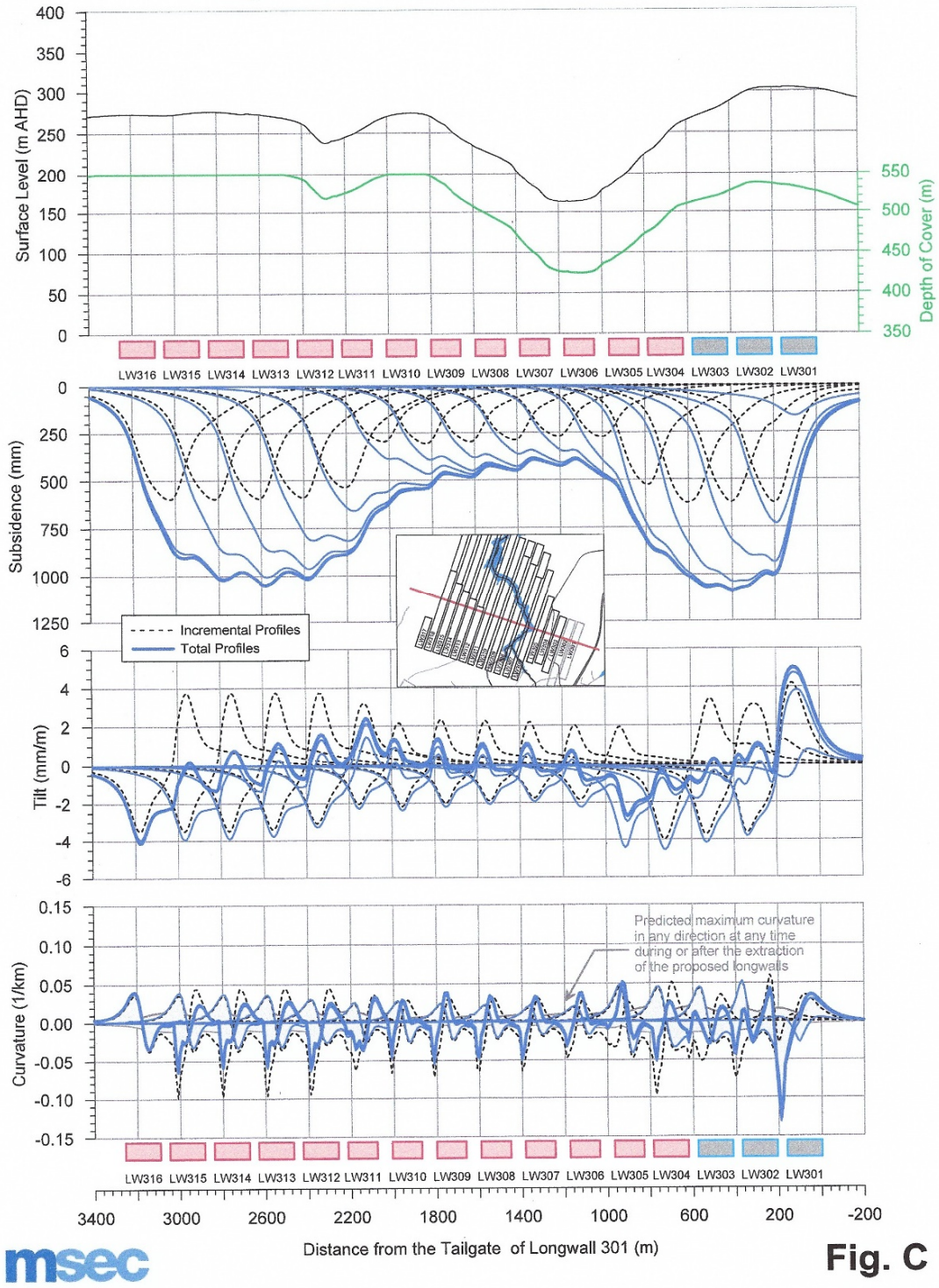
Figure 4.11 Predicted subsidence along a centreline cross-section – LWs 301 to 317 (source: MSEC)
