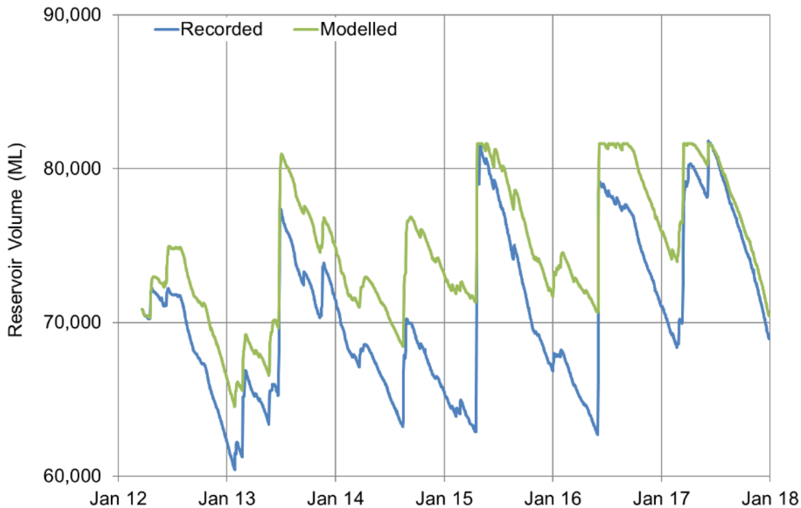
Figure 9 Simulated Reservoir Volume with Systematic Rainfall Error
