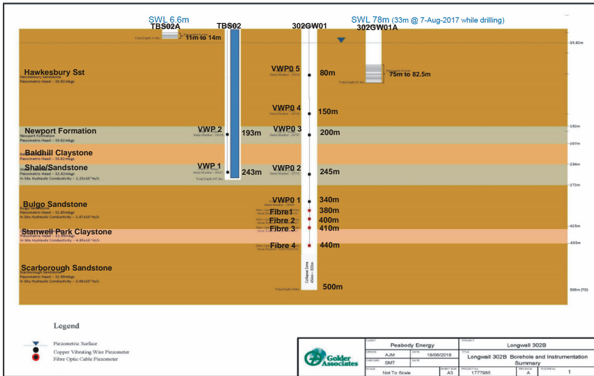
Figure 5.2 Longwall 302 borehole and Instrumentation
