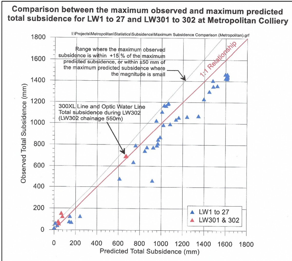
Figure 4.8 MSEC Observed v Predicted subsidence data for Metropolitan Coal
