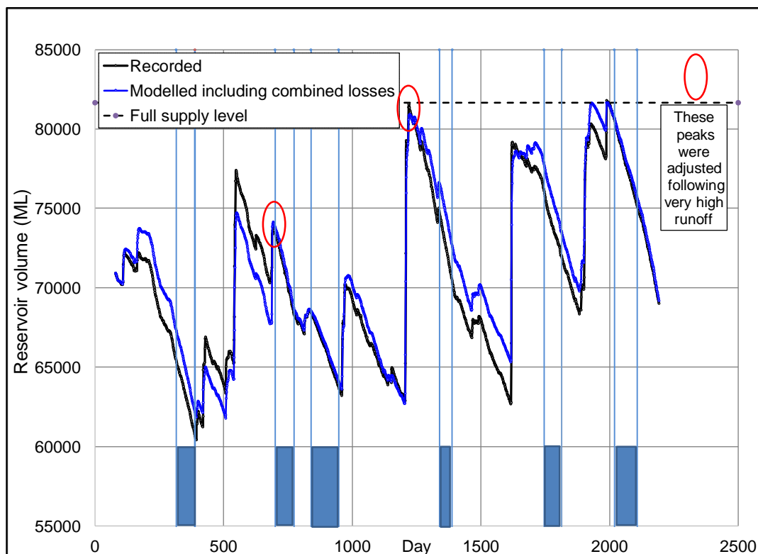
Figure 6.9 Woronora reservoir behaviour diagram for the period 21 Mar 2012 to 31 Dec 2017 for two conditions: (a). Recorded reservoir volume (b) Estimated volumes using water balance model adopting base case inputs and outputs and incorporating a daily combined groundwater loss of 2.9 ML/day and increasing two flood volumes (day 689 by 4900 ML and day 1209 by 3000 ML)
