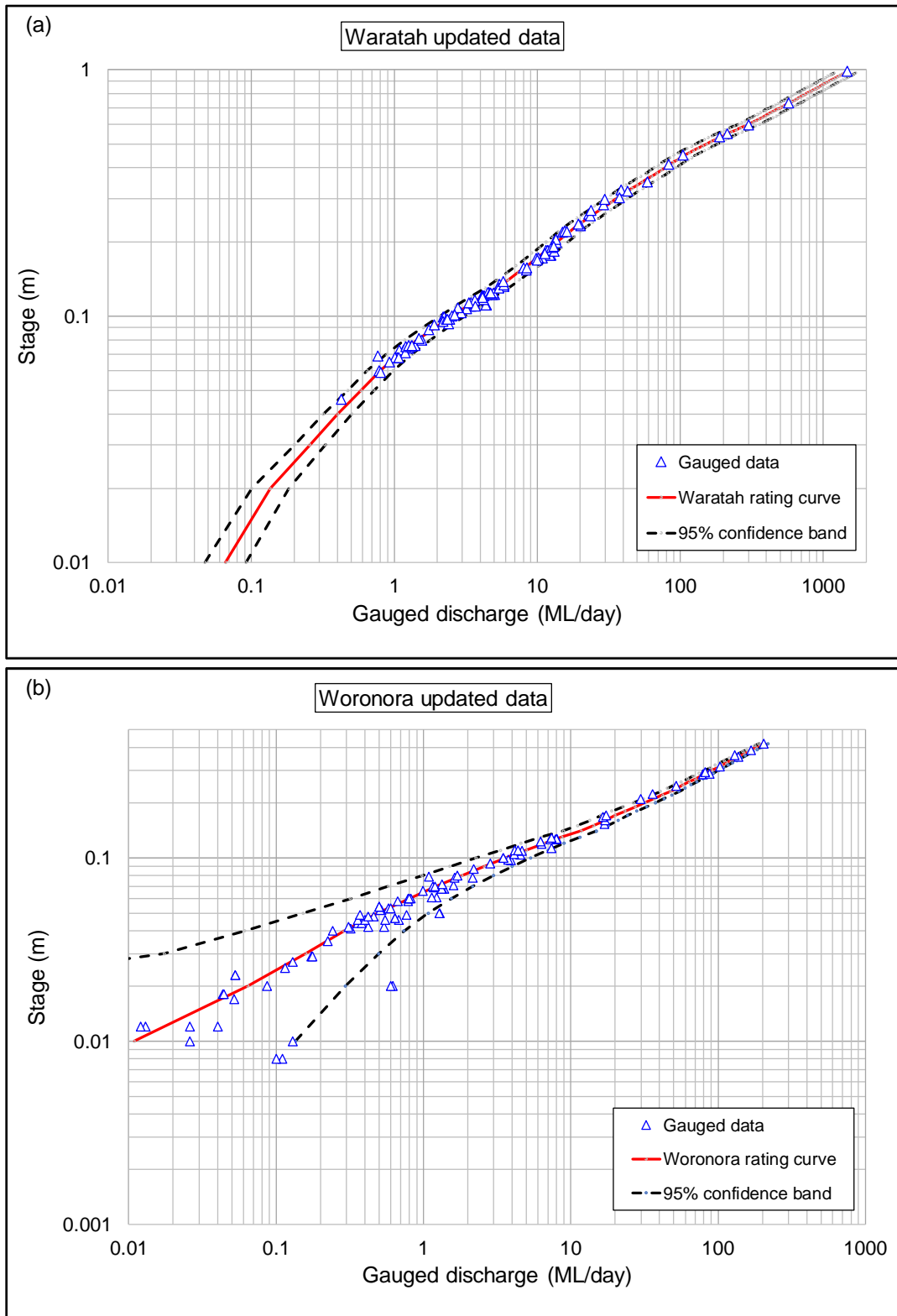
Figure F2. Rating curve for (a) Waratah Rivulet (GS2132102) and (b) Woronora River (GS2132101) showing the 95% uncertainty band
