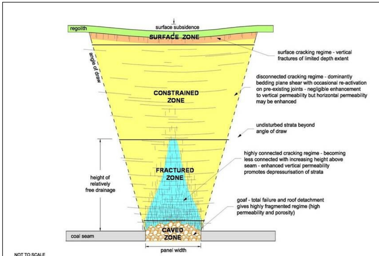
Figure 4.1 “Height of Fracturing” concept. 7
