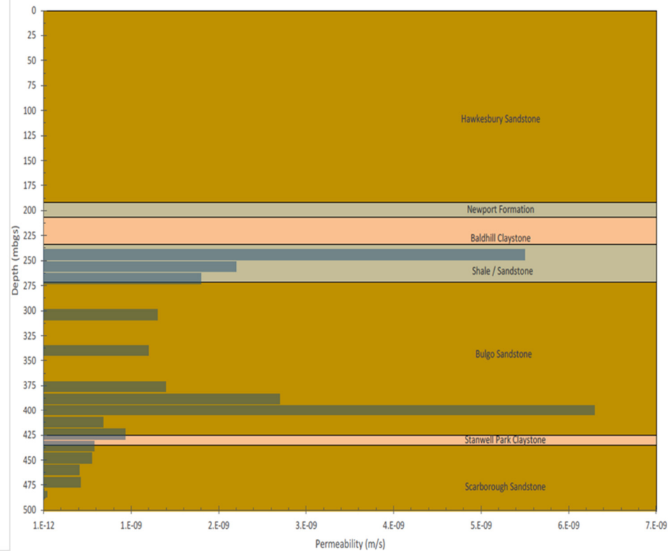
Figure 4.6 LW302 overburden conductivity test results – pre- and post-mining (source: HydroSimulations presentation – February 2019)
