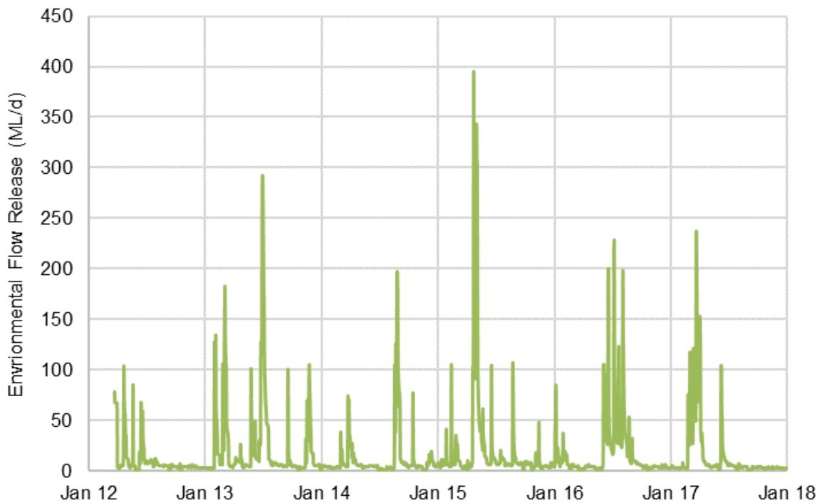
Figure 7 Recorded Environmental Flow Release
