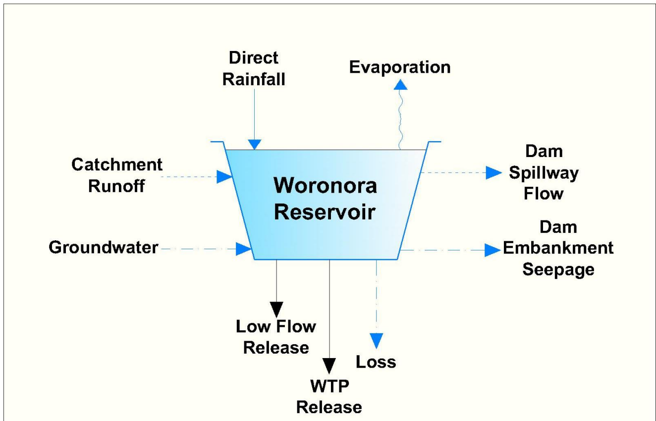
Figure 2 Water Balance Schematic
