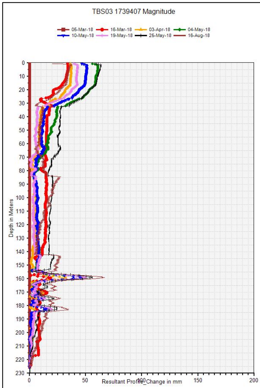
Figure 4.5 Borehole Inclinerometer TBS03 results (source: Golder Longwall 302 TBS02, TBS03 Reports)
