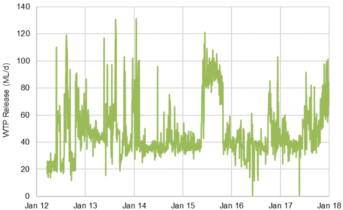
Figure 6 Recorded WTP Release
