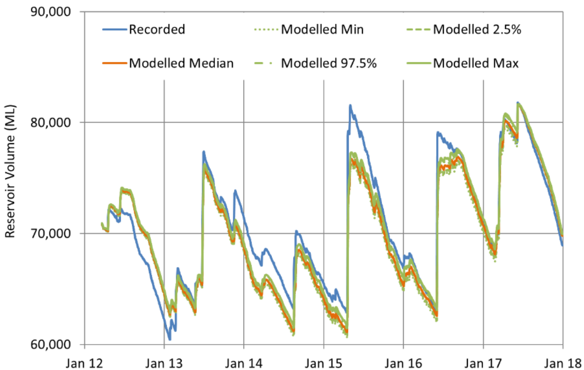
Figure 11 Woronora Reservoir Volume Uncertainty Excluding Ungauged Streamflow Uncertainty
