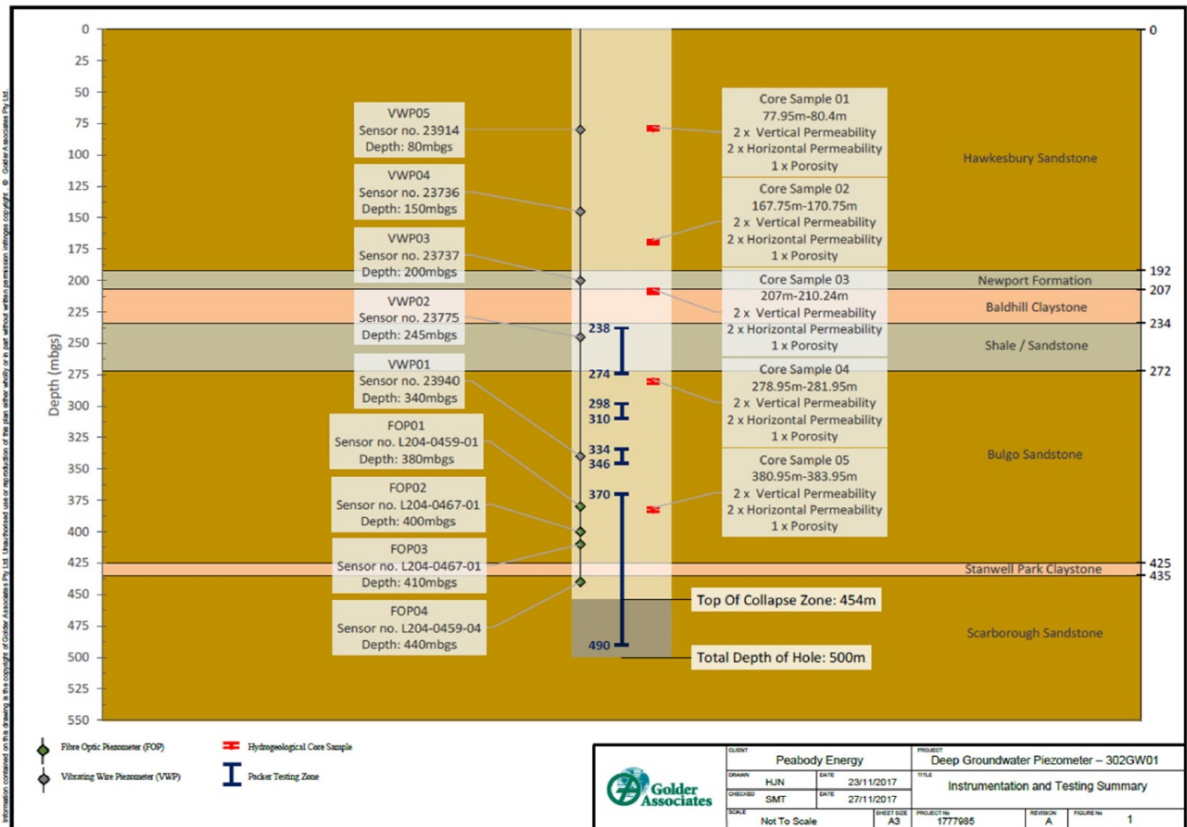
Figure 5.7 Packer tests and Hydraulic conductivities of Core Samples (source: Golder, 2017)
