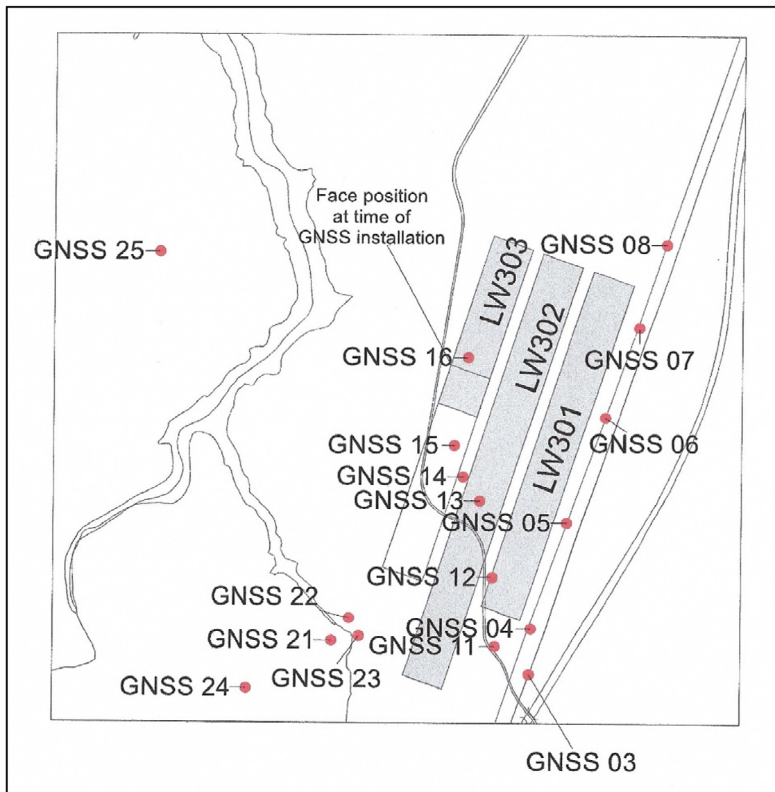
Figure 4.13 GNSS survey station array installed around LWs 301 – 303 (source: MSEC)
