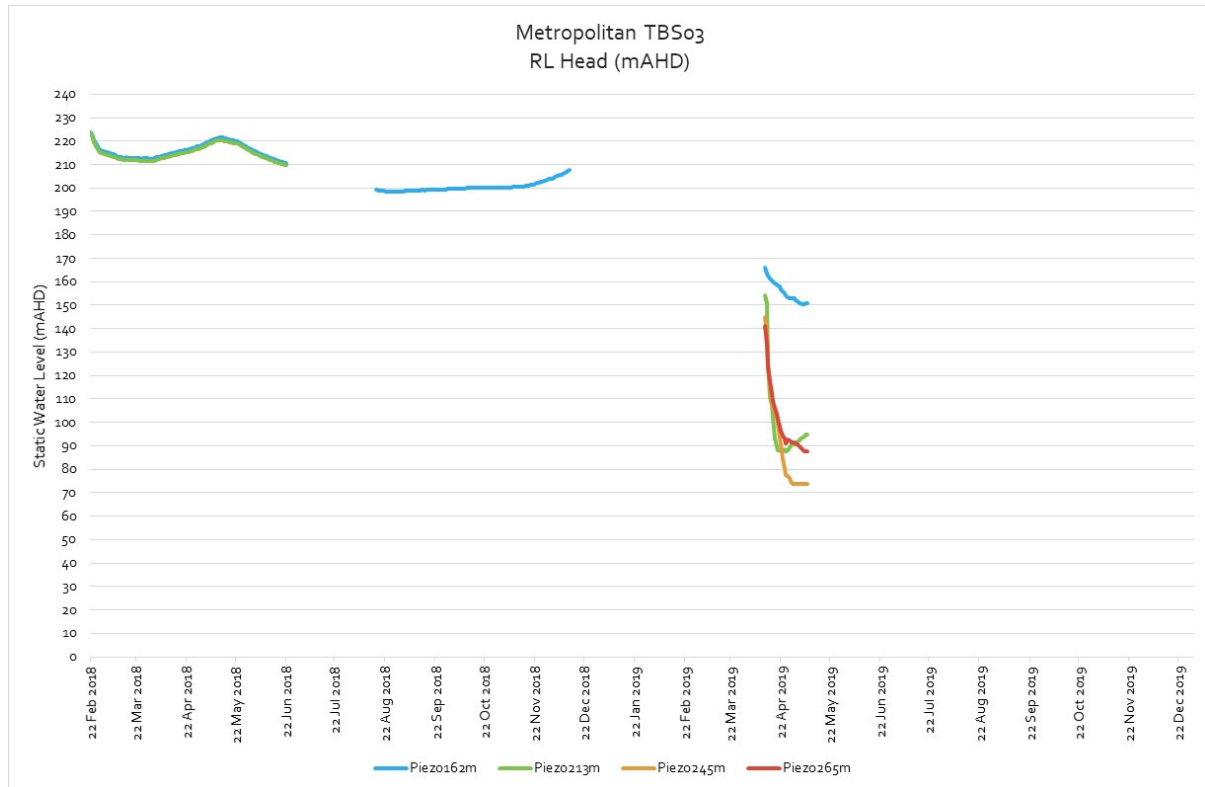
Figure 5.5 TBSO3 piezometer static water levels (source: Metropolitan Coal, 2019)
