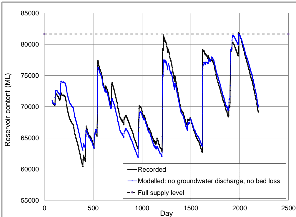
Figure 6.8 Woronora reservoir behaviour diagram for the period 21 Mar 2012 to 31 Dec 2017 for two conditions: (a) Recorded reservoir volume (b) Modelled reservoir volume assuming no combined groundwater loss and Kohler and Parmele lake evaporation increased by 27% (base-case simulation)
