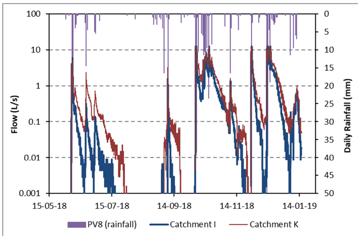
Figure 6.5 Measured hydrographs at flow monitoring stations I and K and observed rainfall at station PV8
