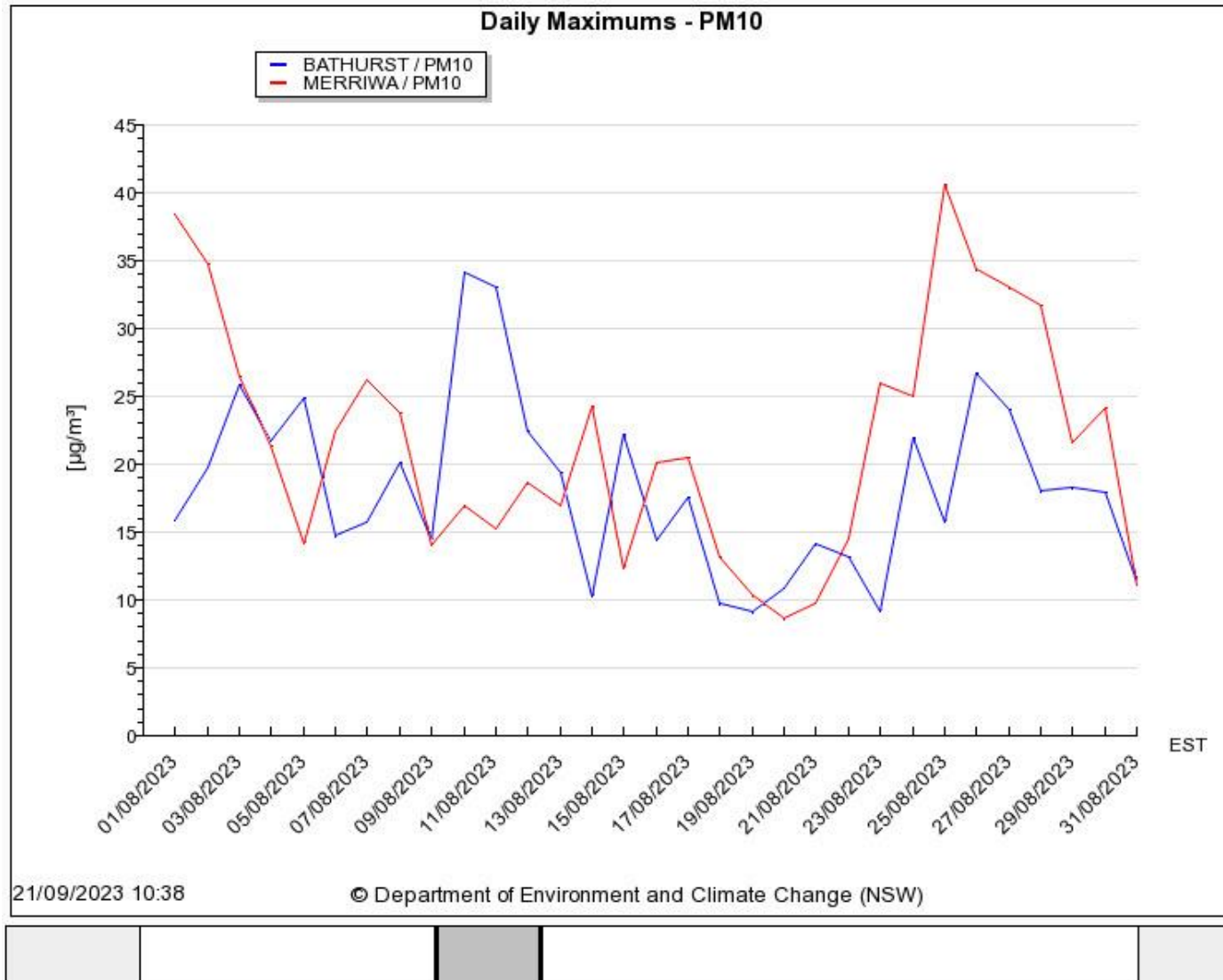
Figure 4. Daily PM10 Average Regional Results
