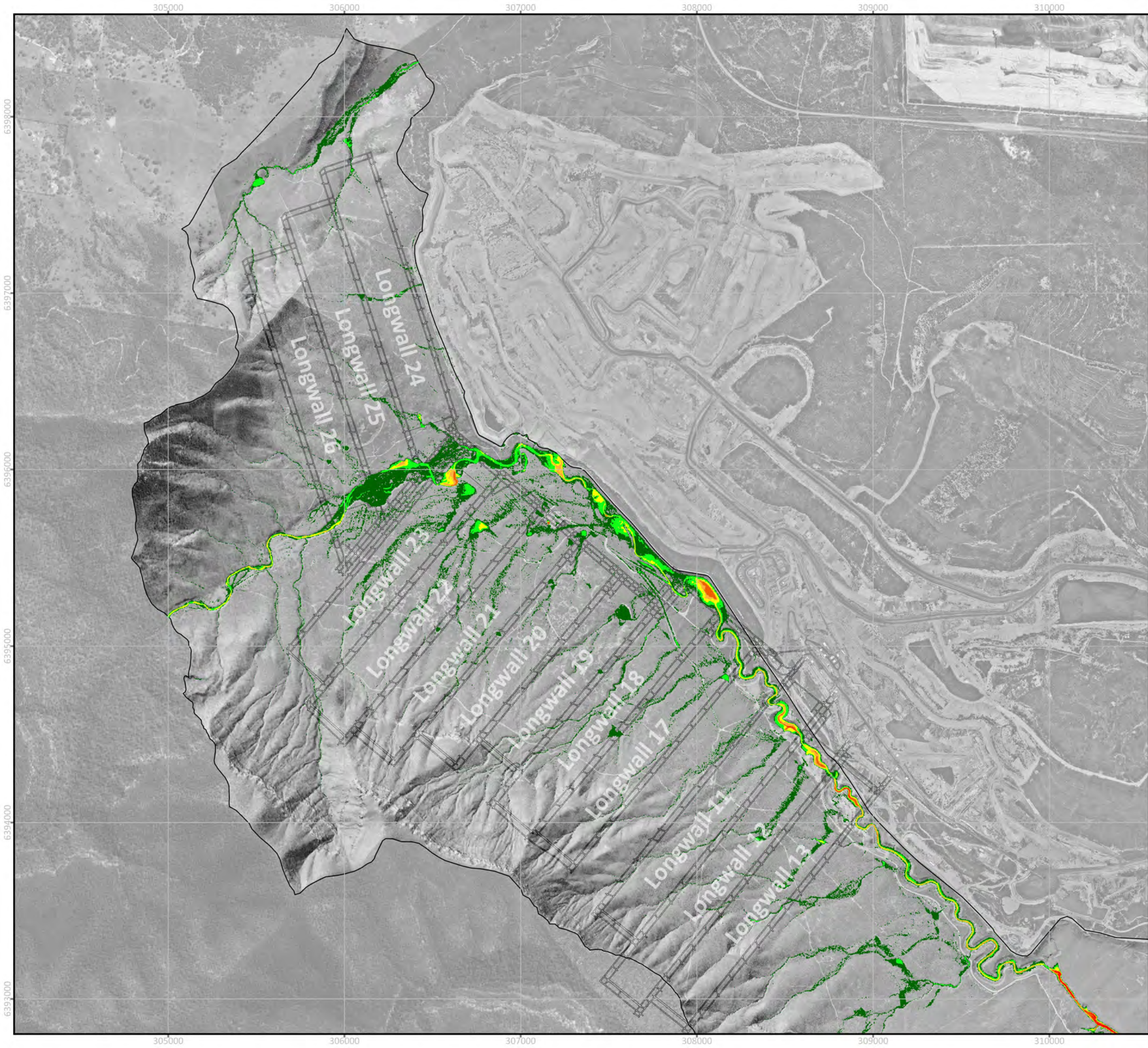
FIGURE C15 0.5 EY EVENT - FLOOD DEPTH SUBSIDED 17-25 SCENARIO PROJECT: 0623002 Wambo Longwall 24-26 Extraction Plan SW
