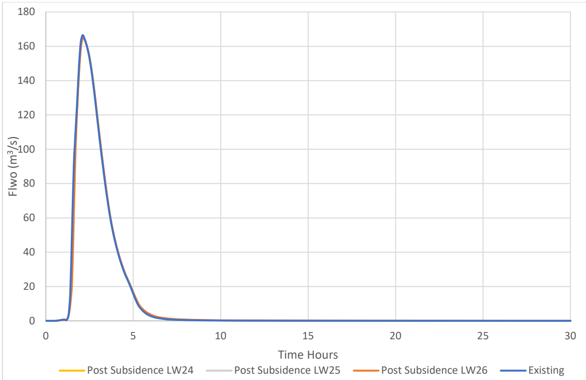
Figure 3-26. North Wambo Creek Hydrograph at FM2 – Pre and post Subsidence (1% AEP Event)
