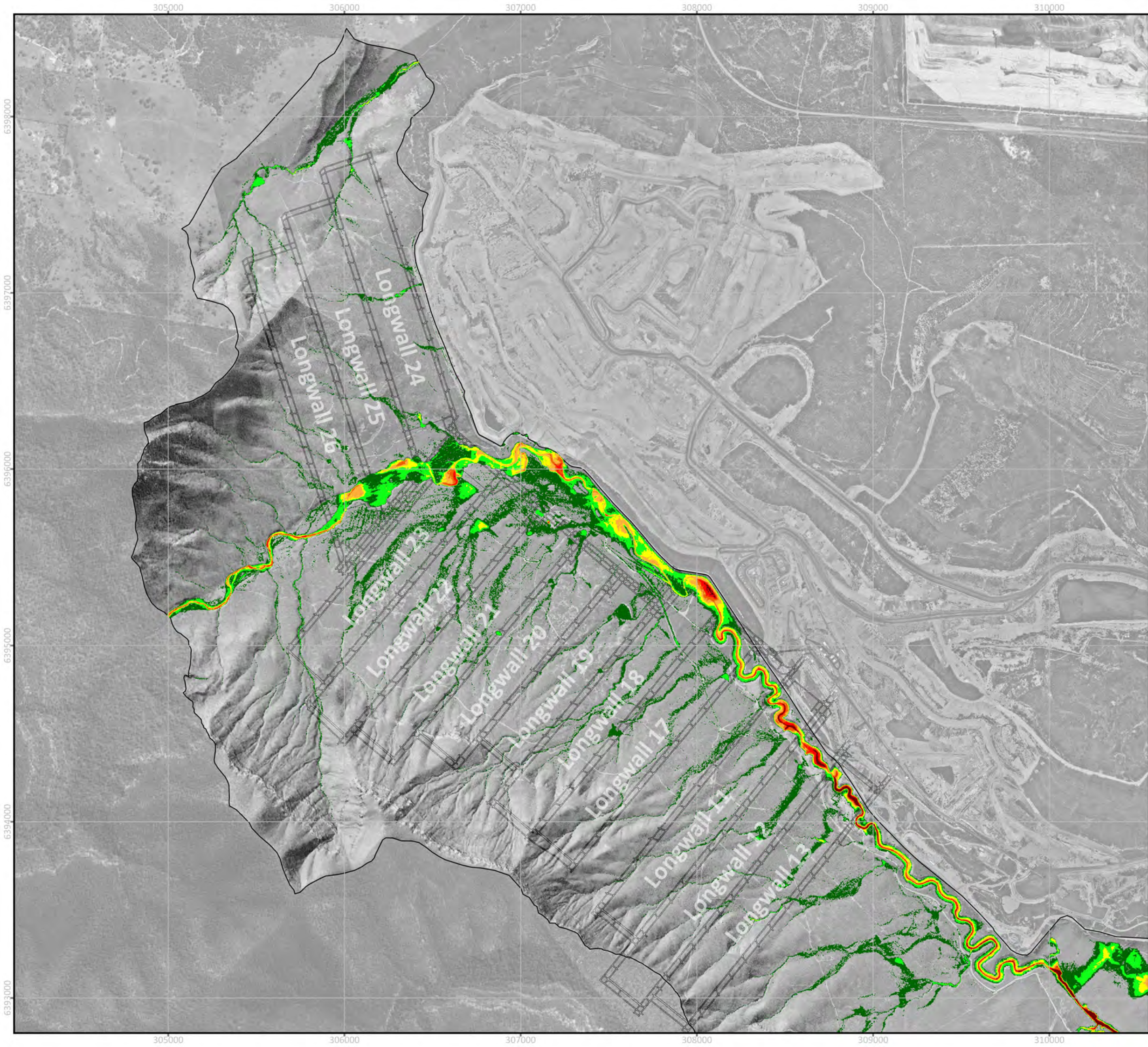
FIGURE C23 2% AEP EVENT - FLOOD DEPTH SUBSIDED 17-26 SCENARIO PROJECT: 0623002 Wambo Longwall 24-26 Extraction Plan SW
