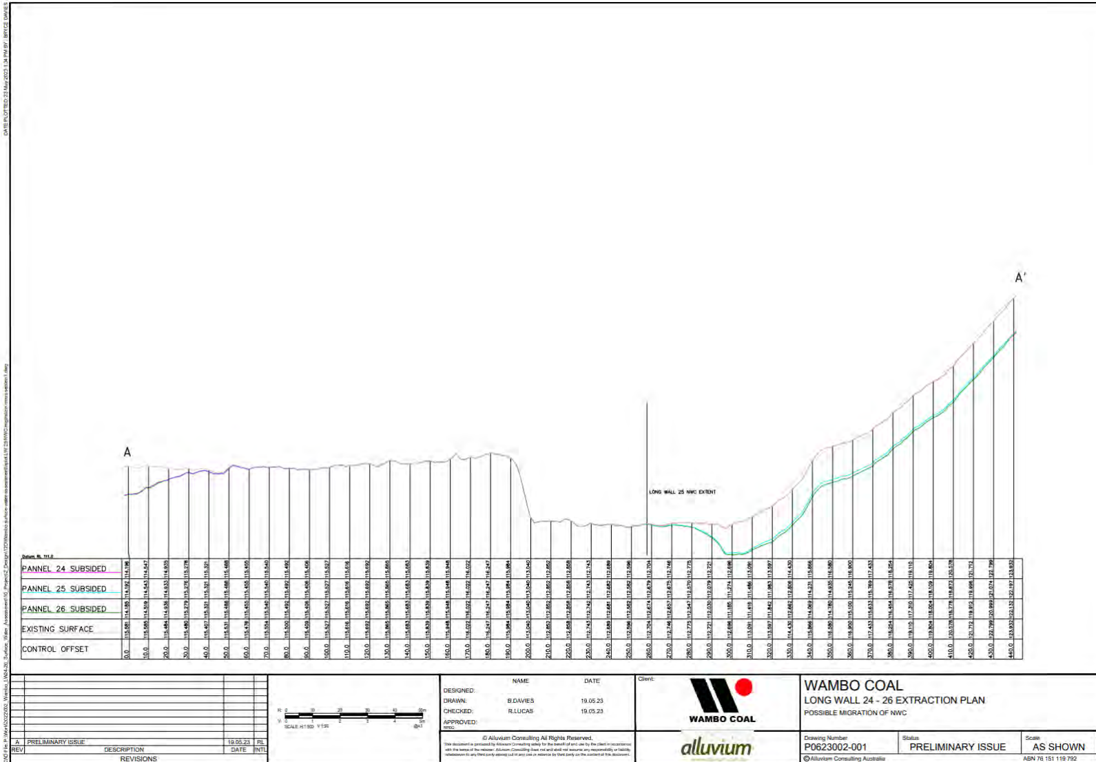
Figure 3-18. Section A-A' Likely North Wambo Creek migration
