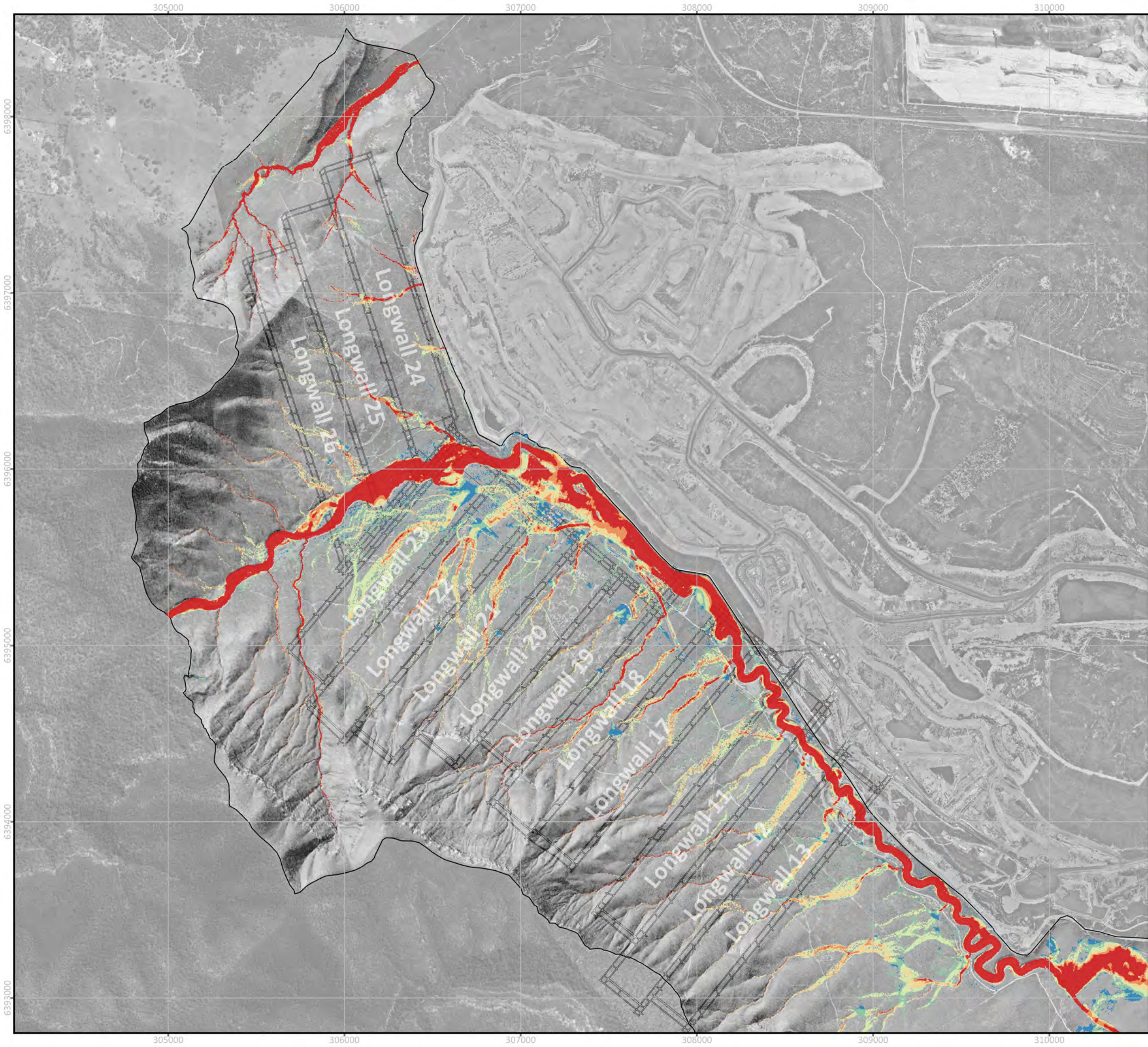
FIGURE C20 0.1% AEP EVENT - FLOOD VELOCITY SUBSIDED 17-25 SCENARIO PROJECT: 0623002 Wambo Longwall 24-26 Extraction Plan SW
