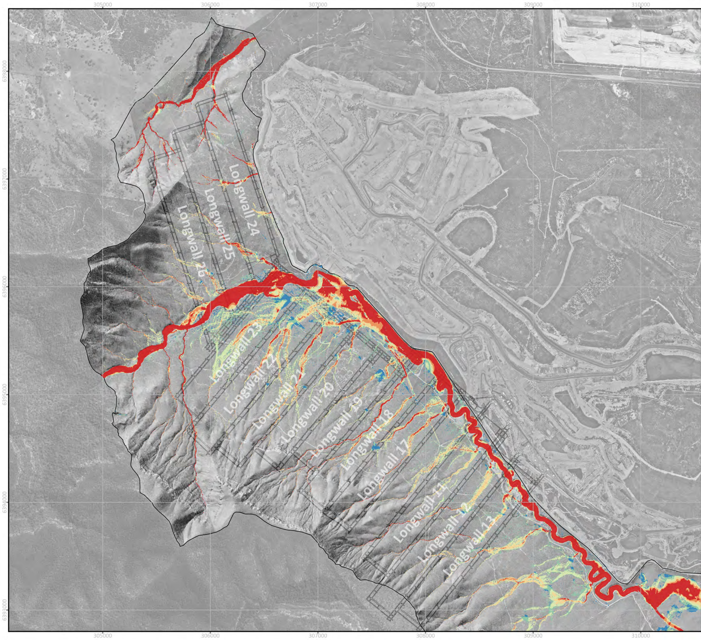
FIGURE C14 0.1% AEP EVENT - FLOOD VELOCITY SUBSIDED 17-24 SCENARIO PROJECT: 0623002 Wambo Longwall 24-26 Extraction Plan SW
