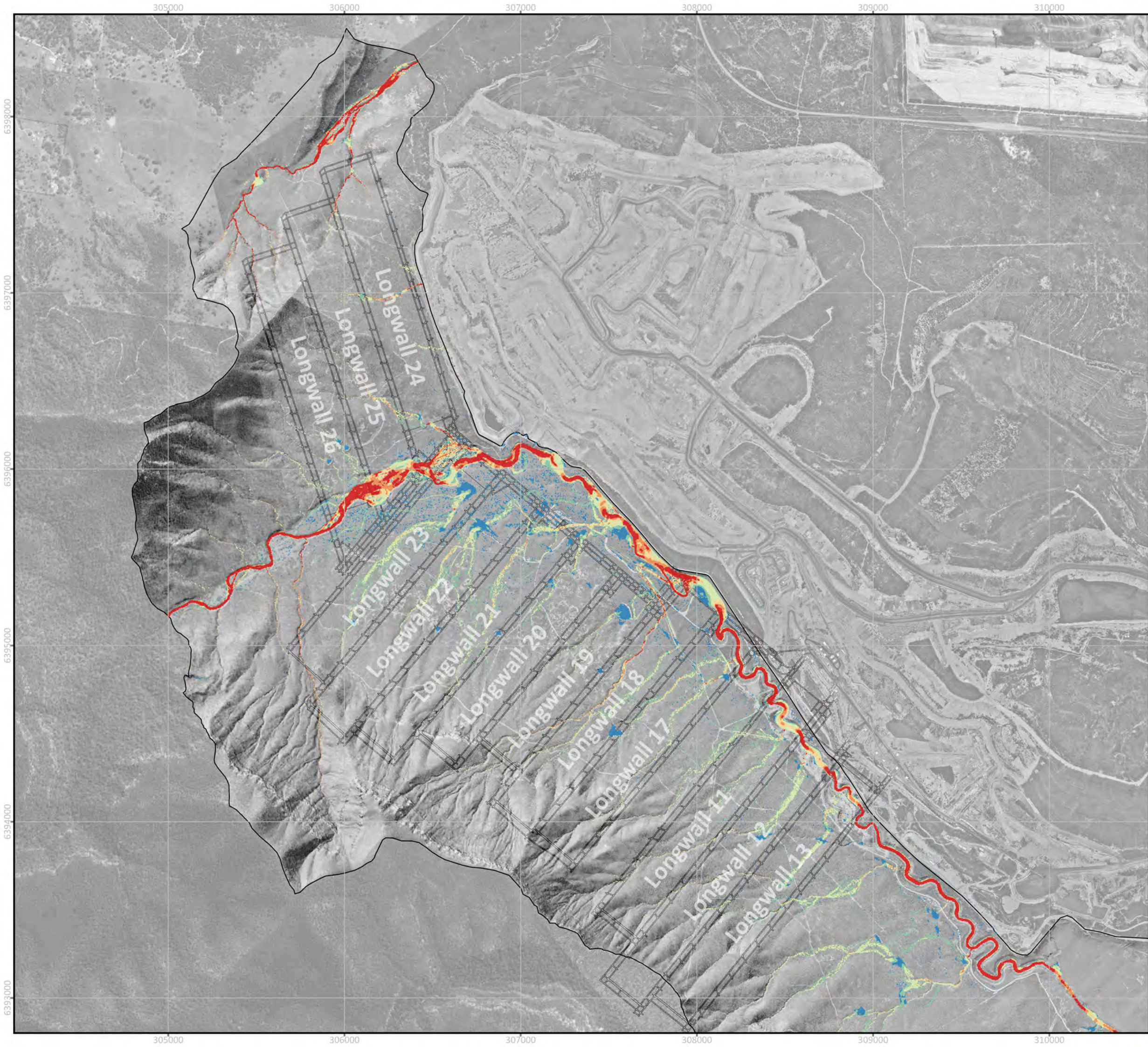
FIGURE C16 0.5 EY EVENT - FLOOD VELOCITY SUBSIDED 17-25 SCENARIO PROJECT: 0623002 Wambo Longwall 24-26 Extraction Plan SW
