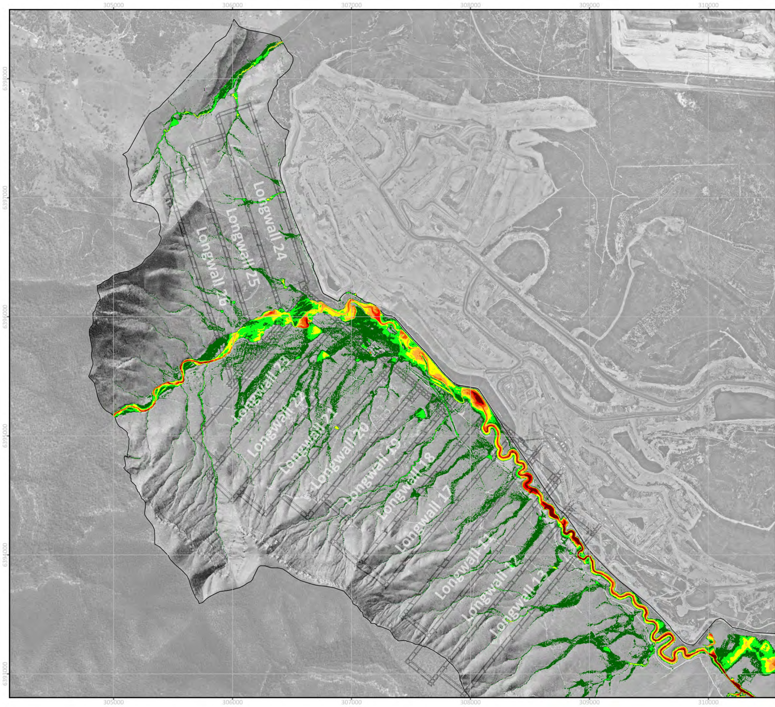
FIGURE C19 0.1% AEP EVENT - FLOOD DEPTH SUBSIDED 17-25 SCENARIO PROJECT: 0623002 Wambo Longwall 24-26 Extraction Plan SW
