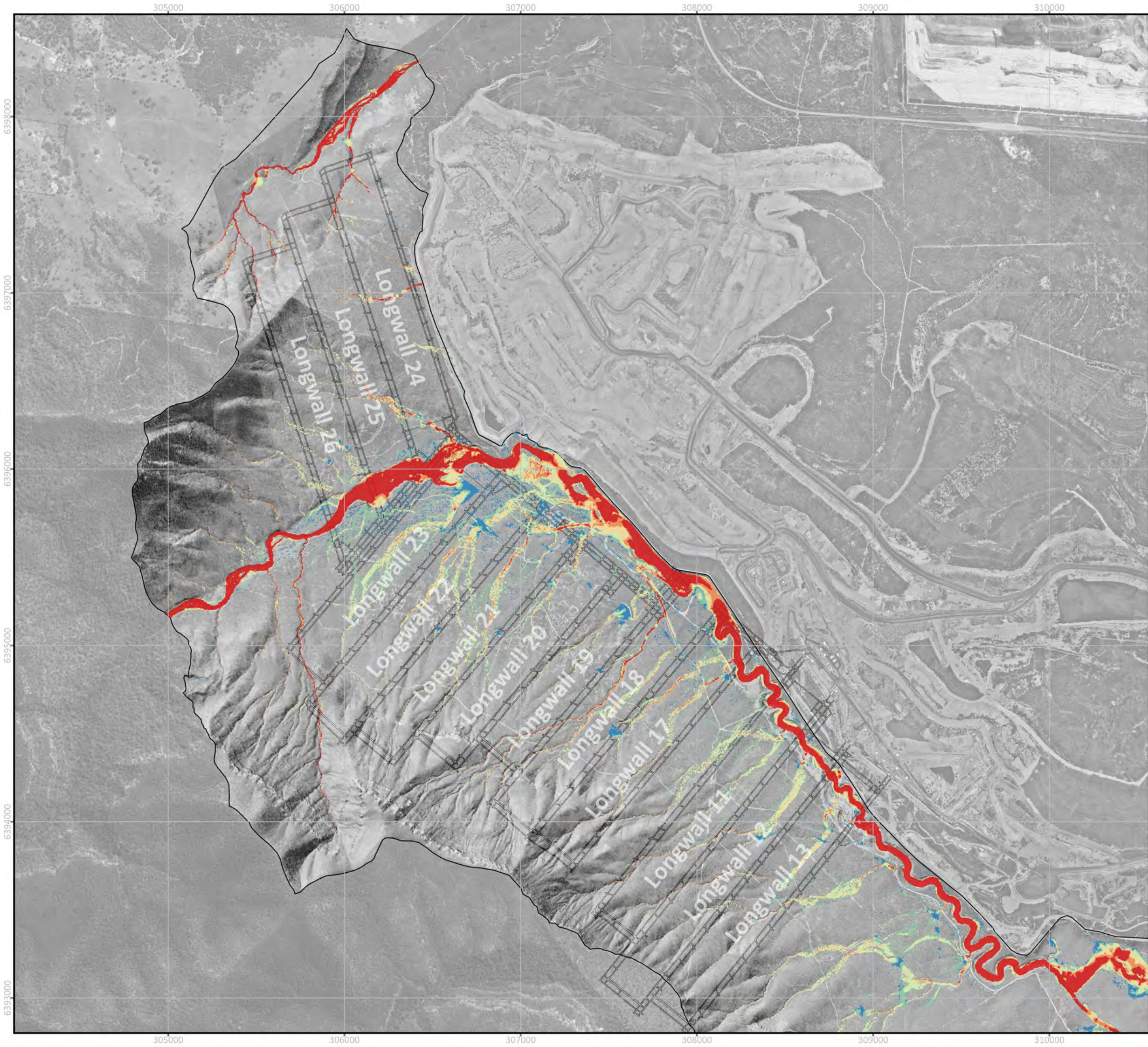
FIGURE C12 2% AEP EVENT - FLOOD VELOCITY SUBSIDED 17-24 SCENARIO PROJECT: 0623002 Wambo Longwall 24-26 Extraction Plan SW
