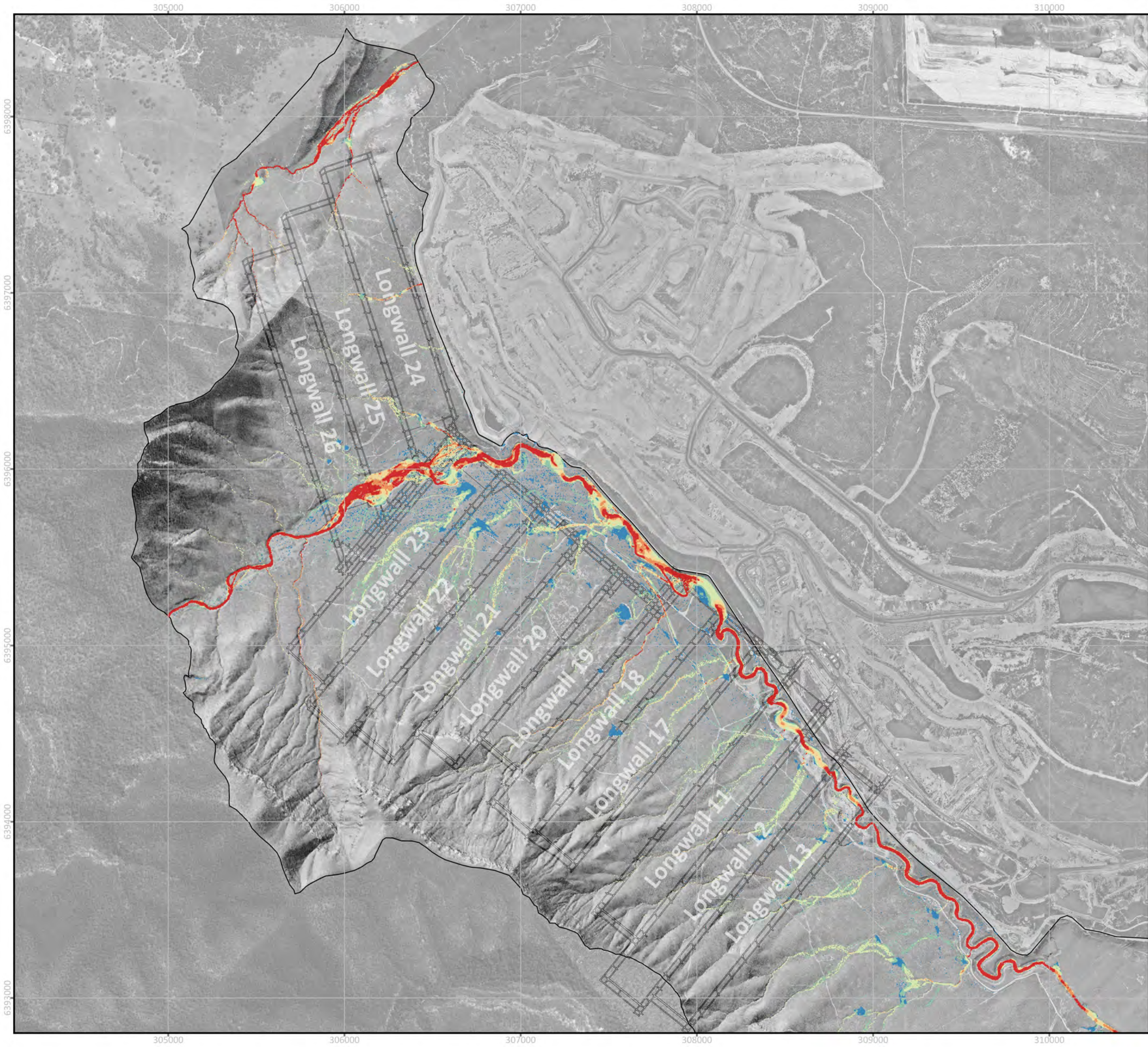
FIGURE C10 0.5 EY EVENT - FLOOD VELOCITY SUBSIDED 17-24 SCENARIO PROJECT: 0623002 Wambo Longwall 24-26 Extraction Plan SW
