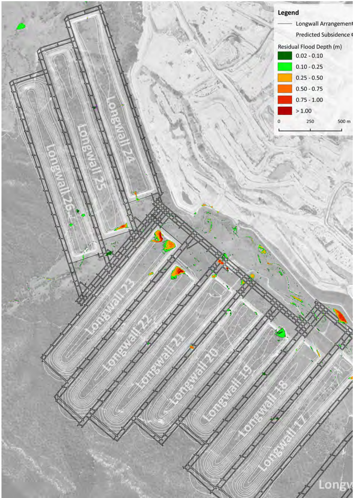
Figure 3-22. 2% AEP Residual Ponding – Longwall 25 Subsided Conditions
