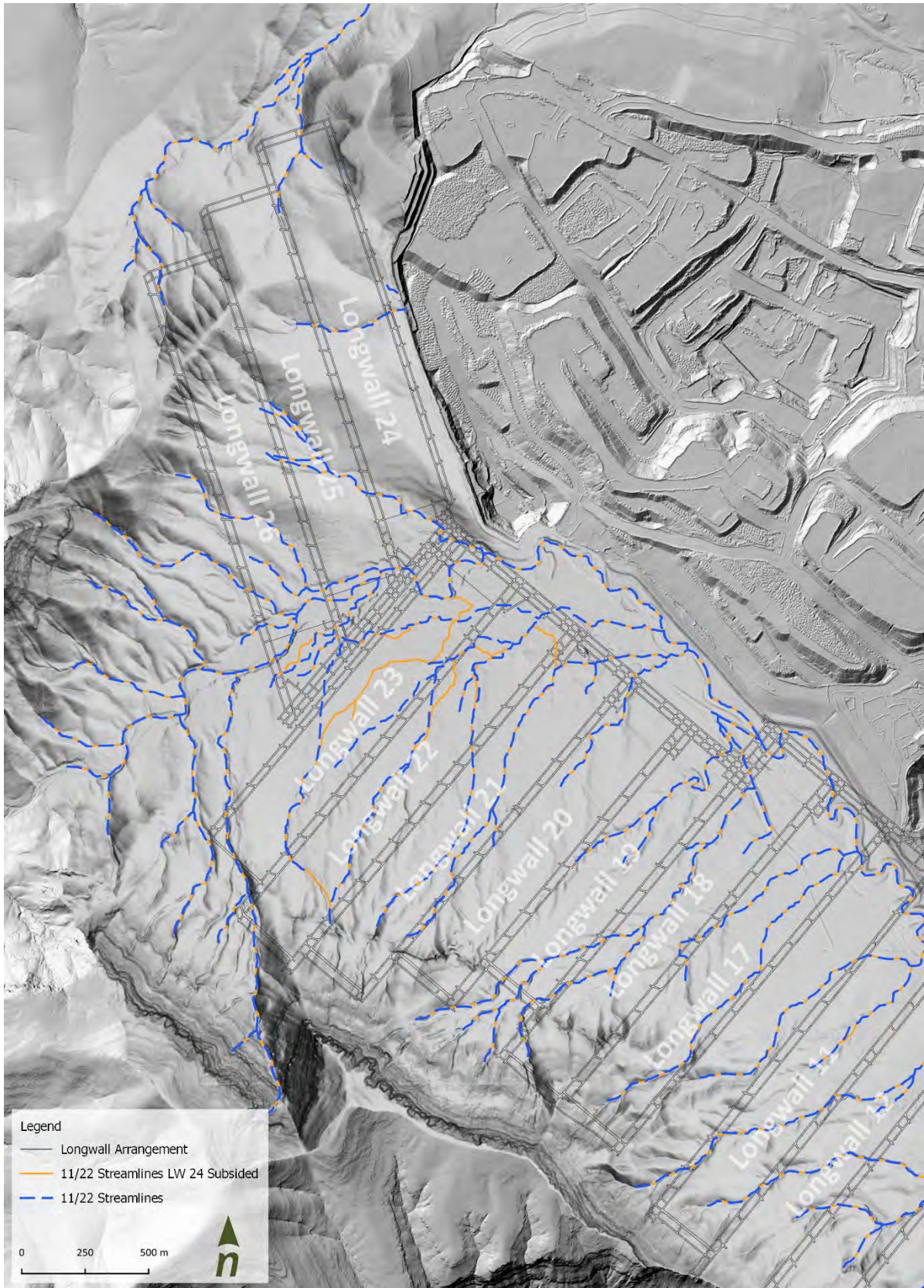
Figure 3-14. Pre and post LW24 Subsidence flow paths (November 2022 lidar)
