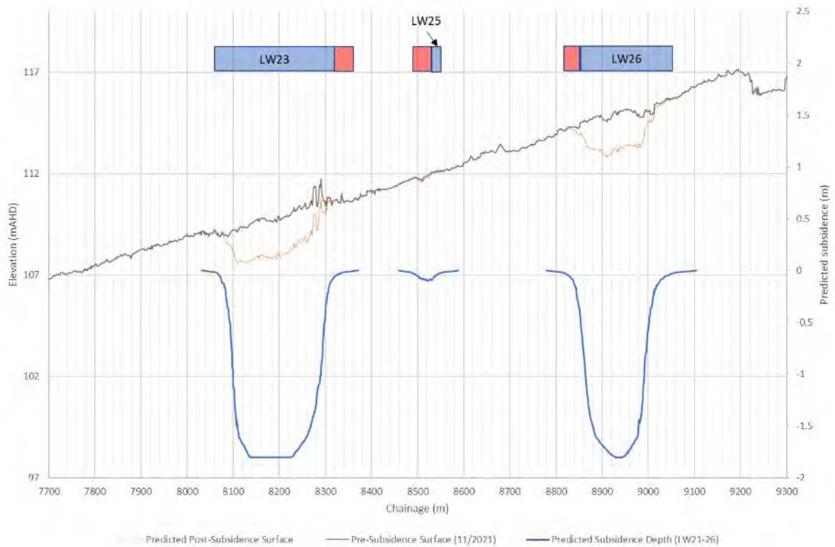
Figure 3-9. Pre and post subsidence longitudinal profile of North Wambo Creek through LW23, LW24 & LW25
