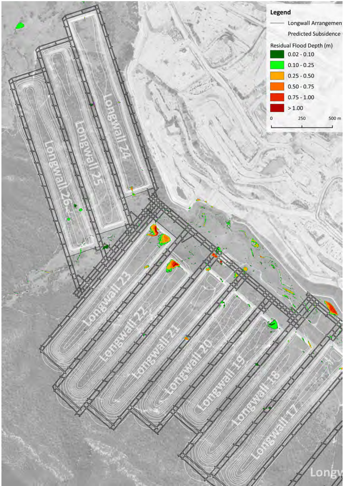
Figure 3-21. 2% AEP Residual Ponding – Longwall 24 Subsided Conditions
