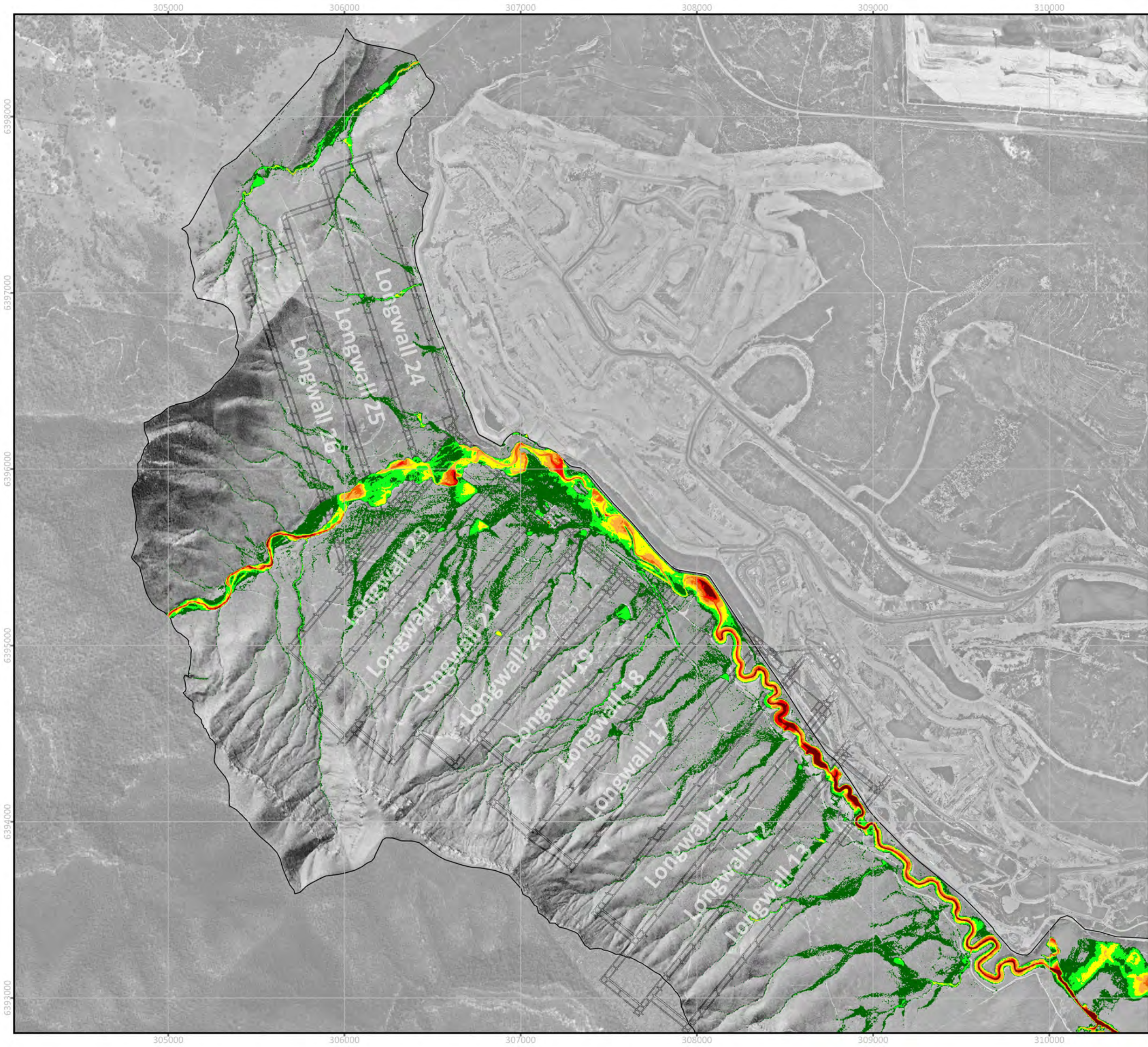
FIGURE C25 0.1% AEP EVENT - FLOOD DEPTH SUBSIDED 17-26 SCENARIO PROJECT: 0623002 Wambo Longwall 24-26 Extraction Plan SW
