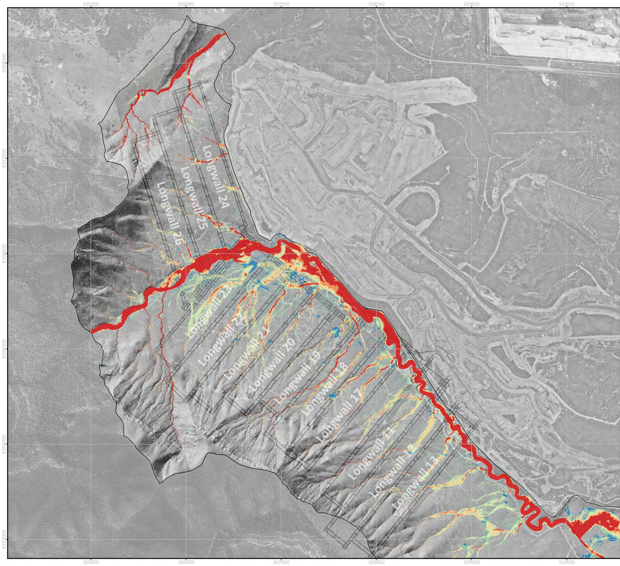
FIGURE C26 0.1% AEP EVENT - FLOOD VELOCITY SUBSIDED 17-26 SCENARIO PROJECT: 0623002 Wambo Longwall 24-26 Extraction Plan SW
