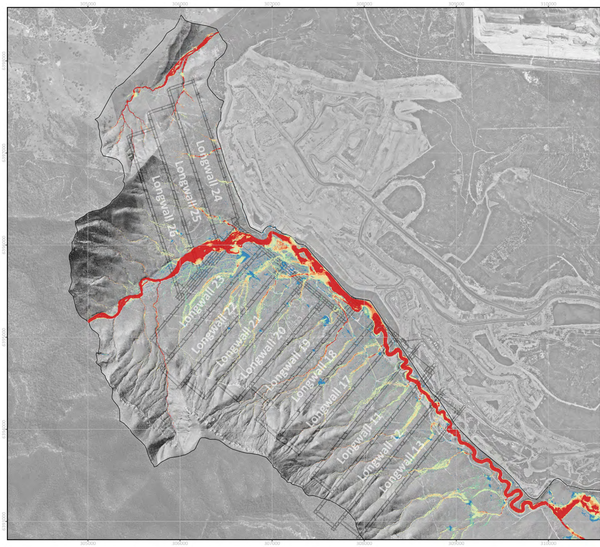
FIGURE C18 2% AEP EVENT - FLOOD VELOCITY SUBSIDED 17-25 SCENARIO PROJECT: 0623002 Wambo Longwall 24-26 Extraction Plan SW
