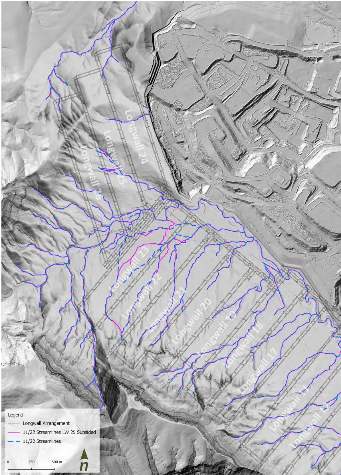
Figure 3-15. Pre and post LW25 Subsidence flow paths (November 2022 lidar)
