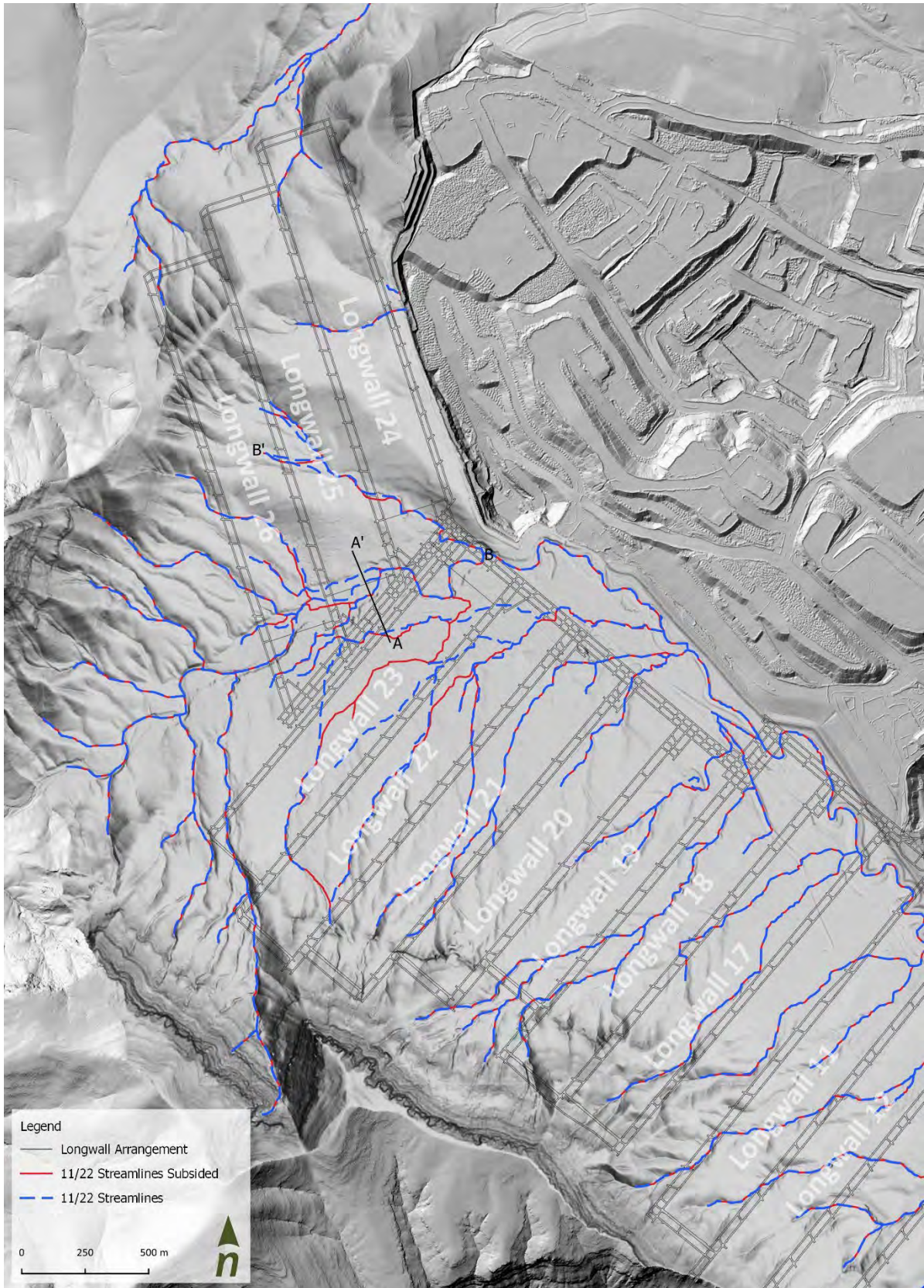
Figure 3-16. Pre and post Subsidence flow paths (November 2022 lidar)
