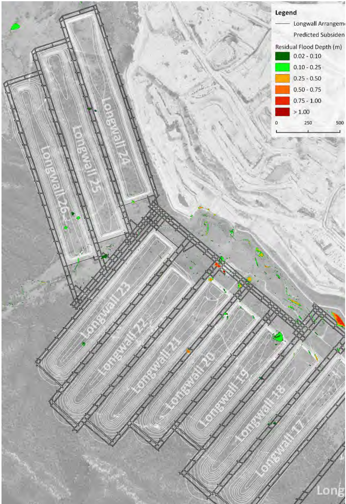
Figure 3-20. 2% AEP Residual Ponding – Existing Conditions
