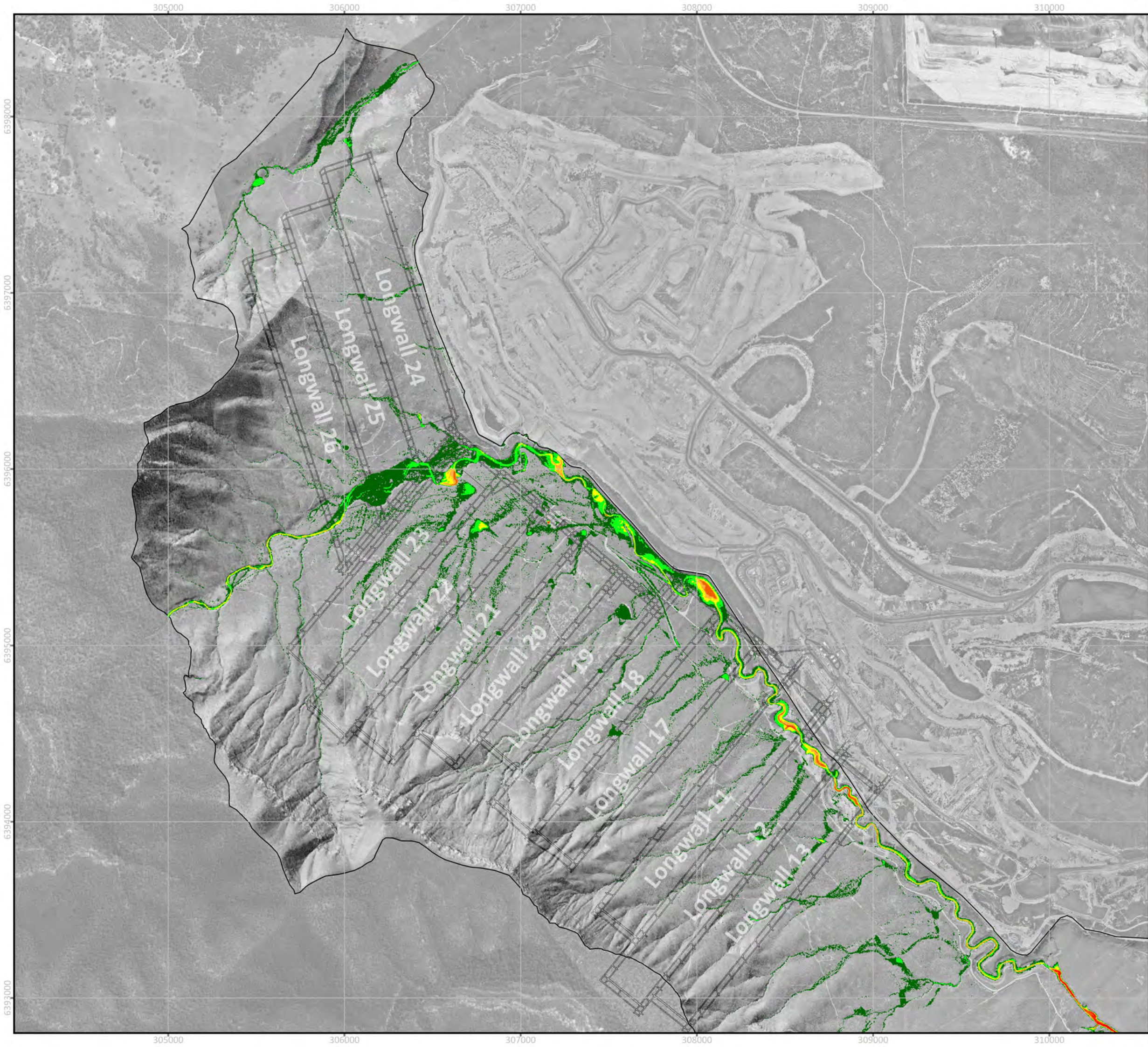
FIGURE C09 0.5 EY EVENT - FLOOD DEPTH SUBSIDED 17-24 SCENARIO PROJECT: 0623002 Wambo Longwall 24-26 Extraction Plan SW
