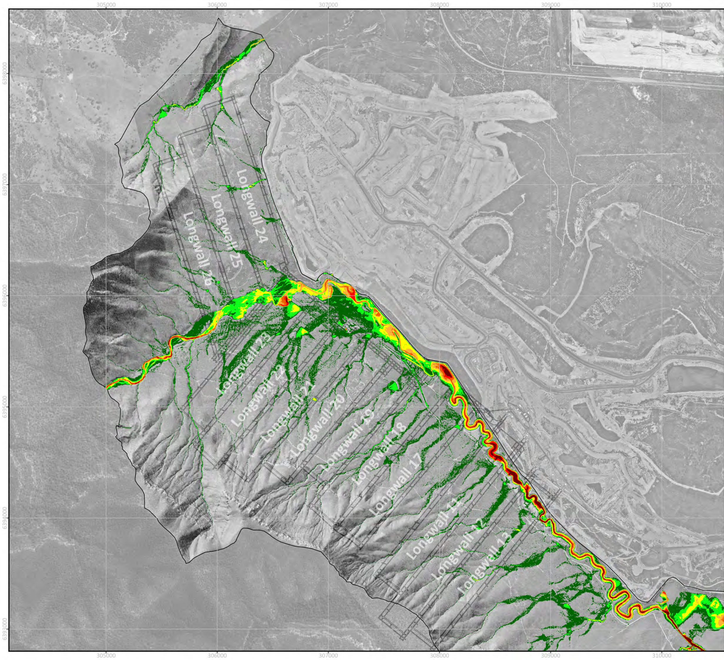
FIGURE C13 0.1% AEP EVENT - FLOOD DEPTH SUBSIDED 17-24 SCENARIO PROJECT: 0623002 Wambo Longwall 24-26 Extraction Plan SW
