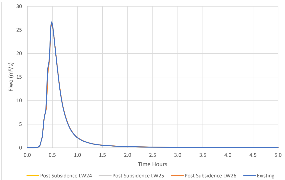
Figure 3-28. Waterfall Creek Hydrograph at downstream of model extent – Pre and post Subsidence (2% AEP Event)
