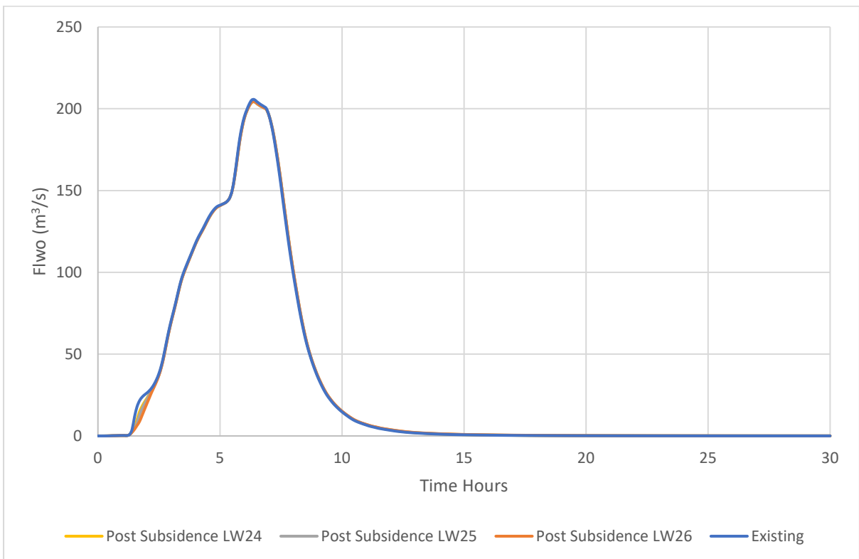
Figure 3-27. North Wambo Creek Hydrograph at FM2 – Pre and post Subsidence (0.1% AEP Event)
