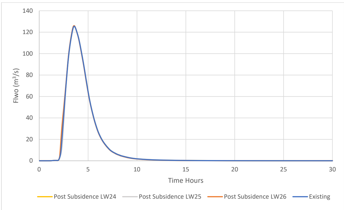
Figure 3-25. North Wambo Creek Hydrograph at FM2 – Pre and post Subsidence (2% AEP Event)
