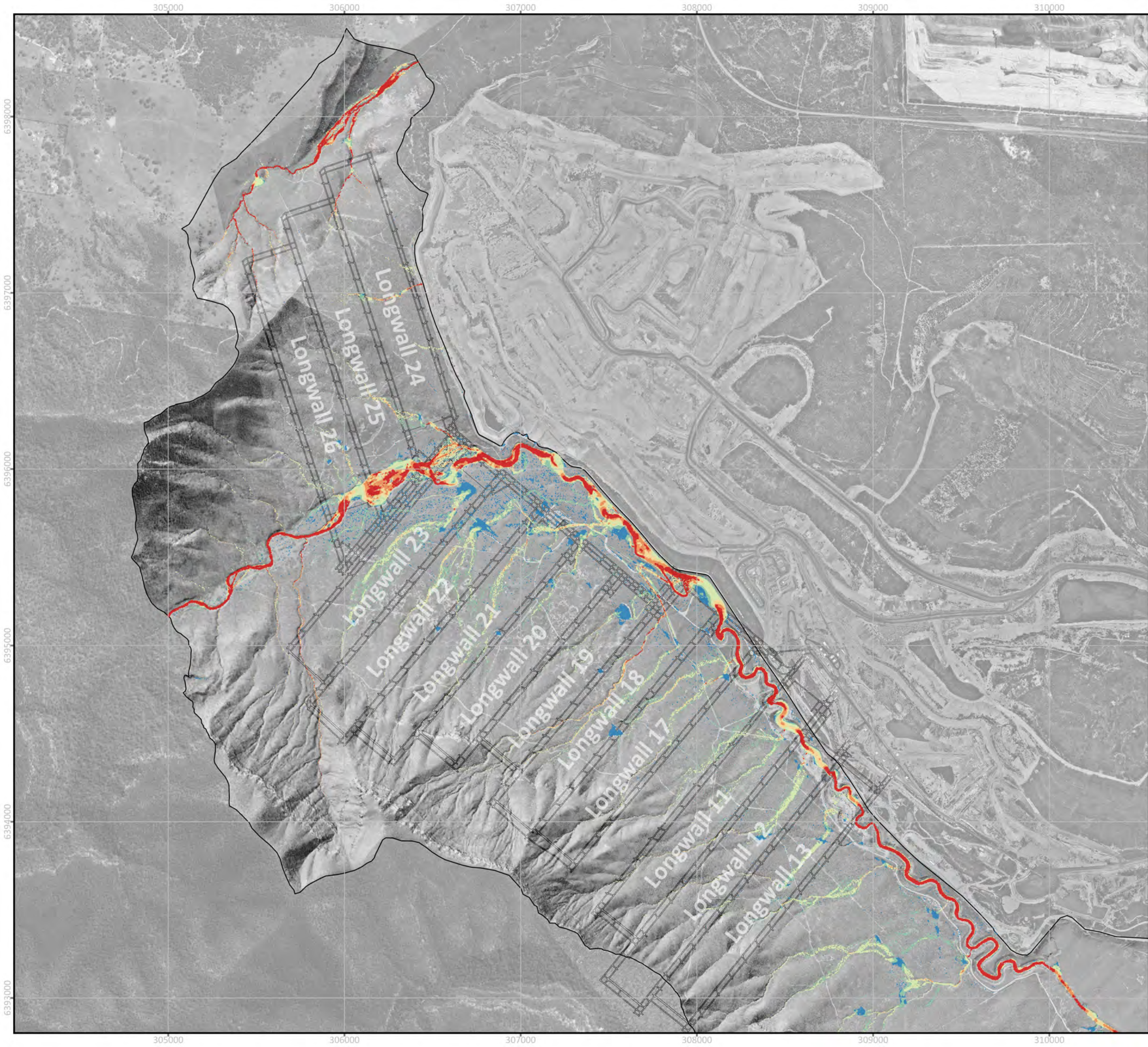
FIGURE C22 0.5 EY EVENT - FLOOD VELOCITY SUBSIDED 17-26 SCENARIO PROJECT: 0623002 Wambo Longwall 24-26 Extraction Plan SW
