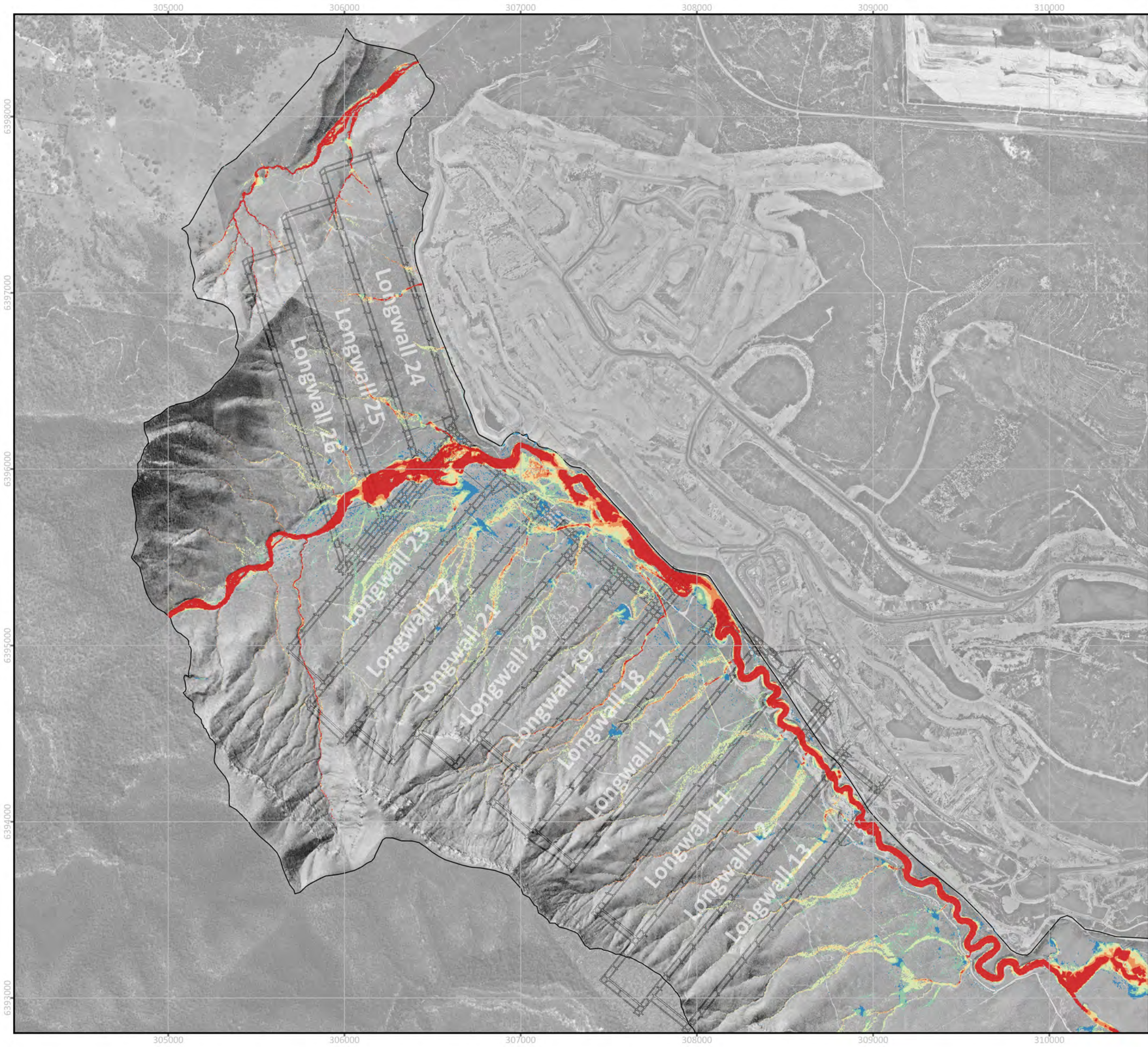
FIGURE C24 2% AEP EVENT - FLOOD VELOCITY SUBSIDED 17-26 SCENARIO PROJECT: 0623002 Wambo Longwall 24-26 Extraction Plan SW
