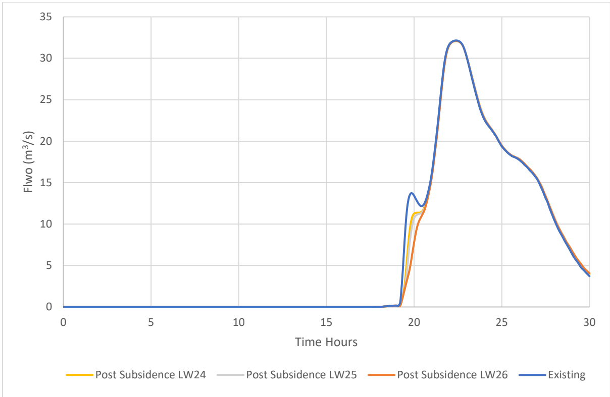
Figure 3-24. North Wambo Creek Hydrograph at FM2 – Pre and post Subsidence (0.5EY Event)
