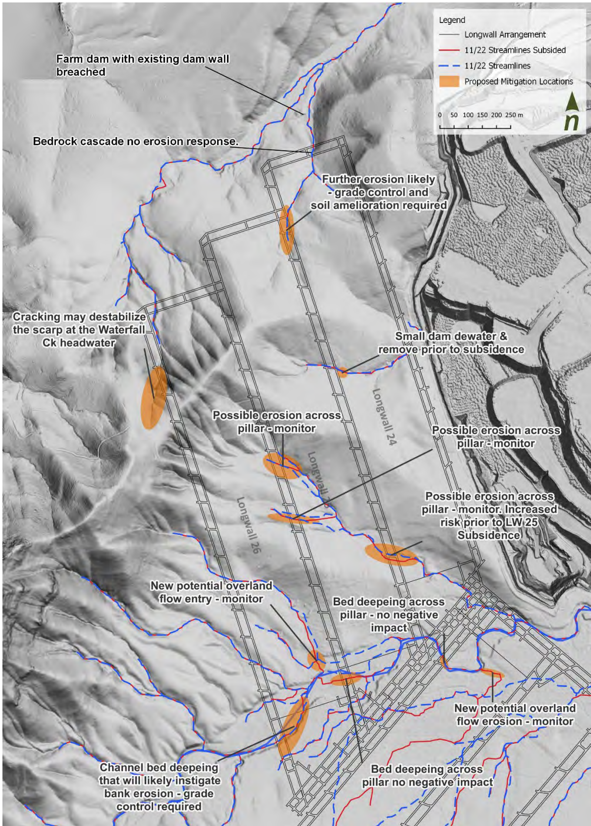
Figure 4-3. Locations where mitigation measures are likely required following subsidence
