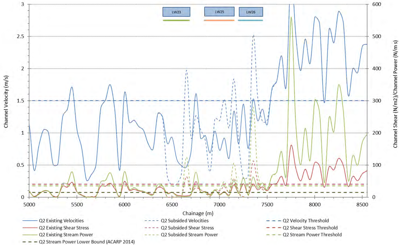
Figure 3-13. Existing and post subsidence hydraulic conditions for 0.5EY Event (1 in 2 AEP) zoomed in to area of interest
