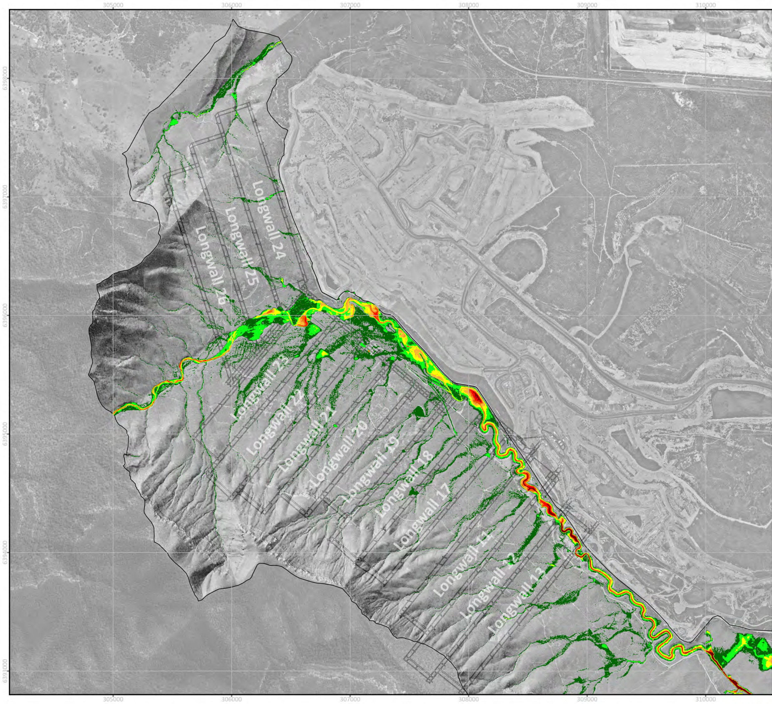
FIGURE C17 2% AEP EVENT - FLOOD DEPTH SUBSIDED 17-25 SCENARIO PROJECT: 0623002 Wambo Longwall 24-26 Extraction Plan SW
