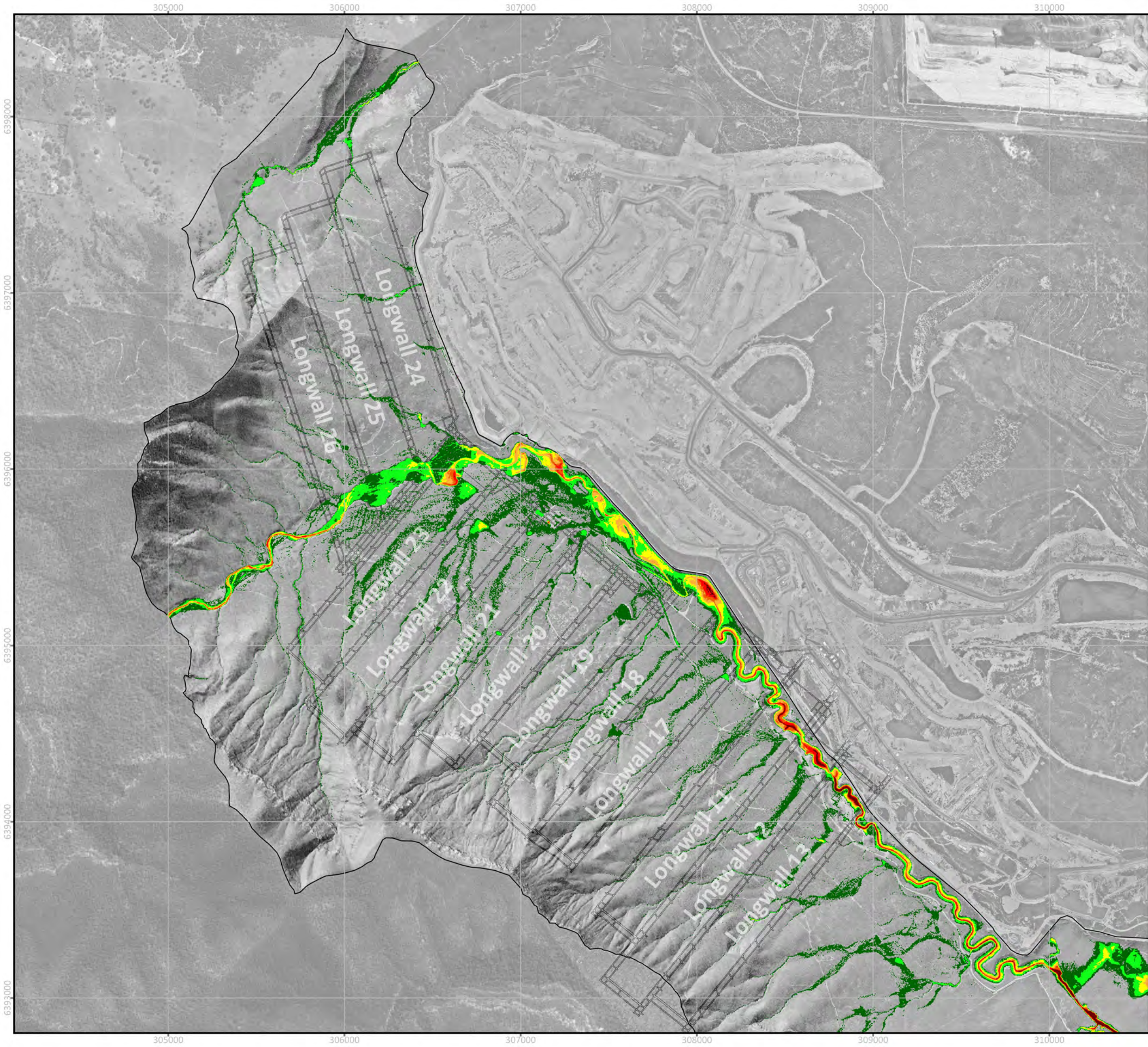
FIGURE C11 2% AEP EVENT - FLOOD DEPTH SUBSIDED 17-24 SCENARIO PROJECT: 0623002 Wambo Longwall 24-26 Extraction Plan SW
