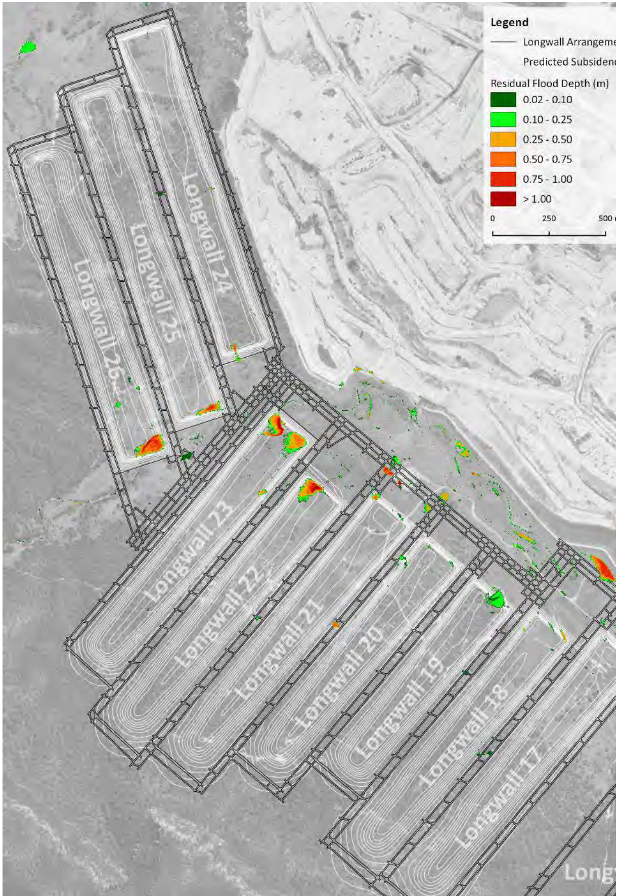
Figure 3-23. 2% AEP Residual Ponding – Longwall 26 Subsided Conditions
