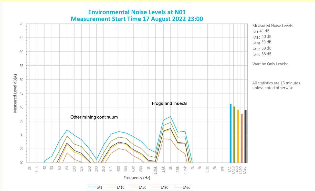
Figure 5.2 Environmental Noise Levels, N01 – Wambo Road
