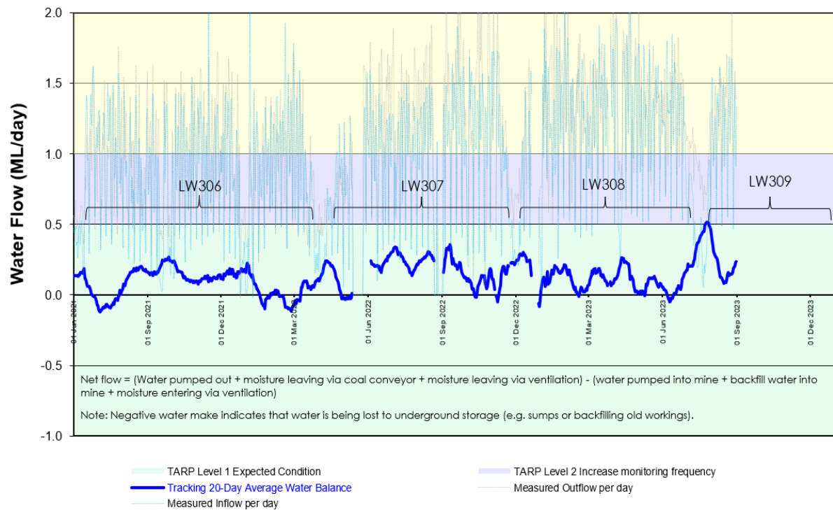
Chart 3b Estimated Daily Mine Water Make, January 2020 to August 2023
