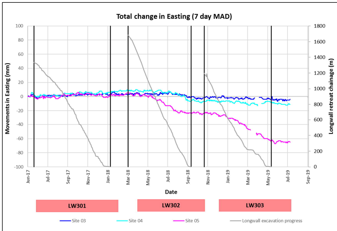
Figure 6: Movements in Easting at Sites GNSS03, GNSS04 and GNSS05
