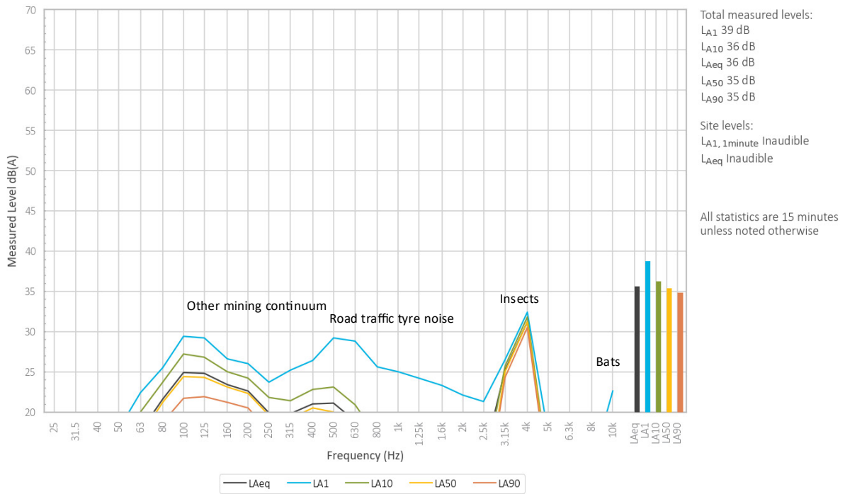
Figure 5.3 Environmental noise levels, N16 – Jerrys Plains Road
