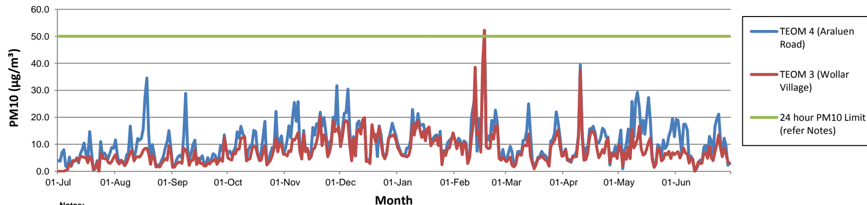
Figure 3. TEOM (PM10) Results - 12 Month Trend
