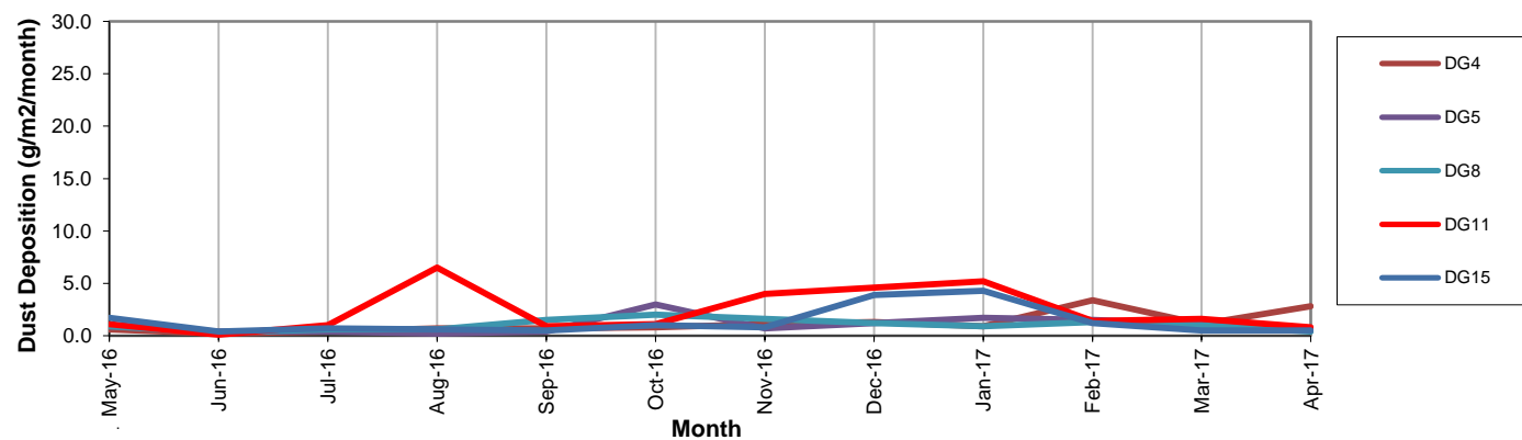
Figure 1a. DG Results - 12 Month Trend
