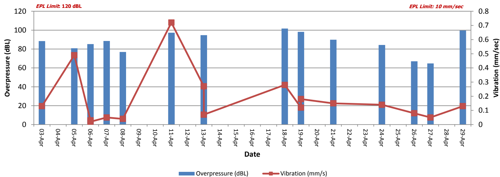
Figure 7. Overpressure (dBL) and Vibration (mm/sec) recorded during Month
