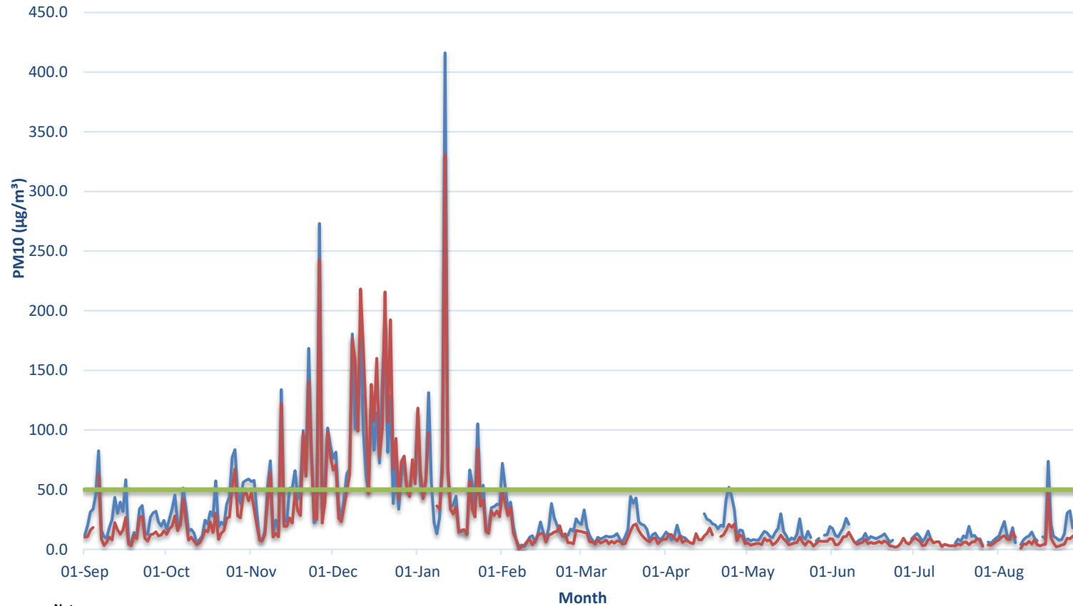
Figure 3. TEOM (PM10) Results - 12 Month Trend
