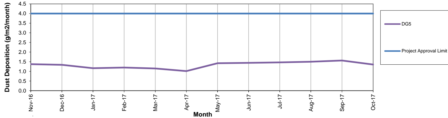
Figure 1b. DG 5 Results - Annual Average
