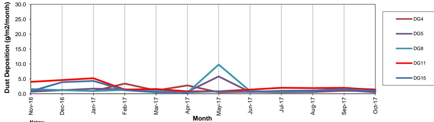
Figure 1a. DG Results - 12 Month Trend
