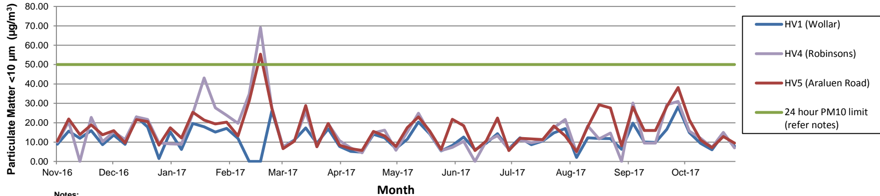
Figure 2. HV (PM10) Results - 12 Month Trend
