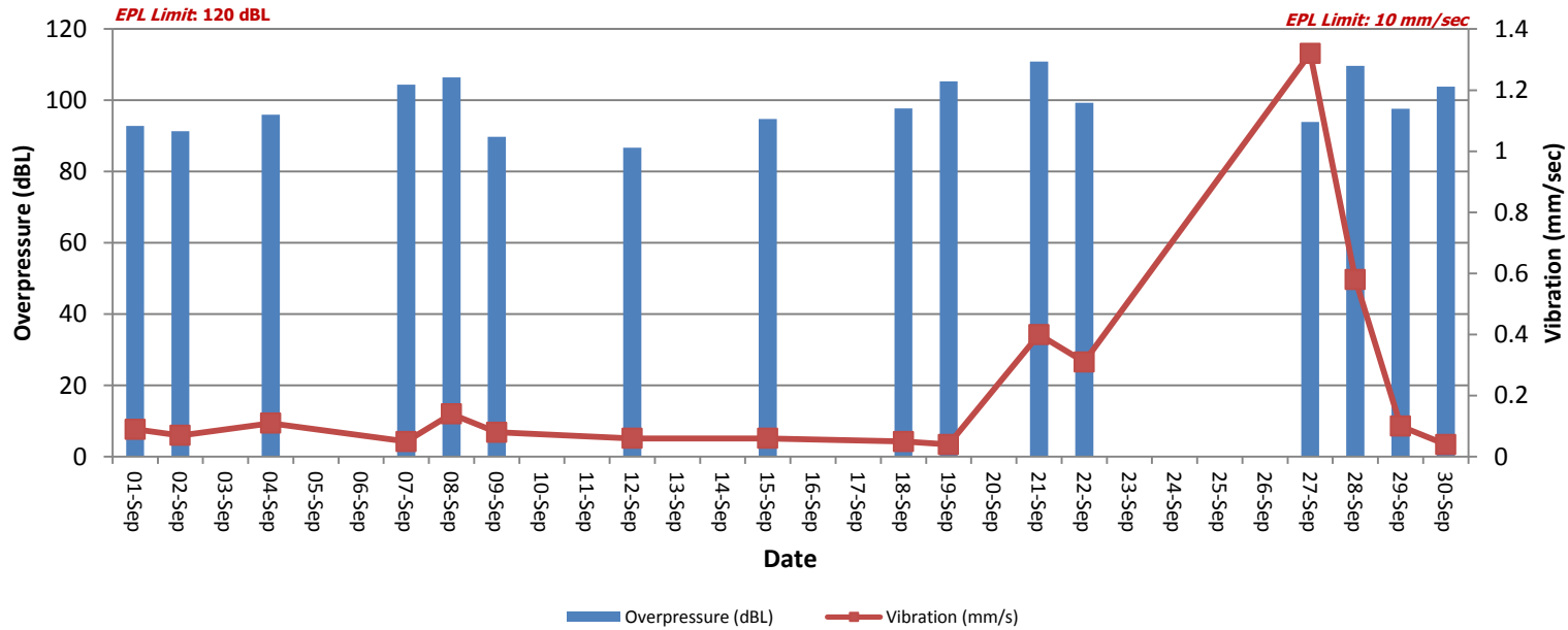
Figure 4. Overpressure (dBL) and Vibration (mm/sec) recorded during Month
