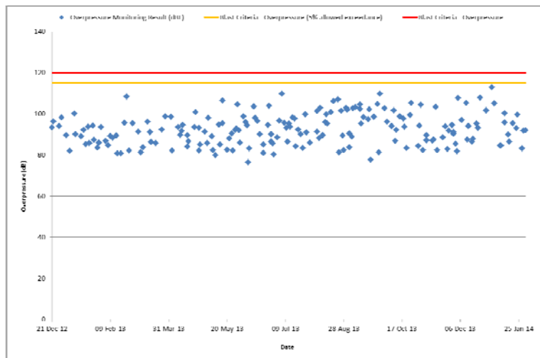
Figure 4: Historical Monitoring Results – Wollar Public School (2012-2014) – Overpressure
