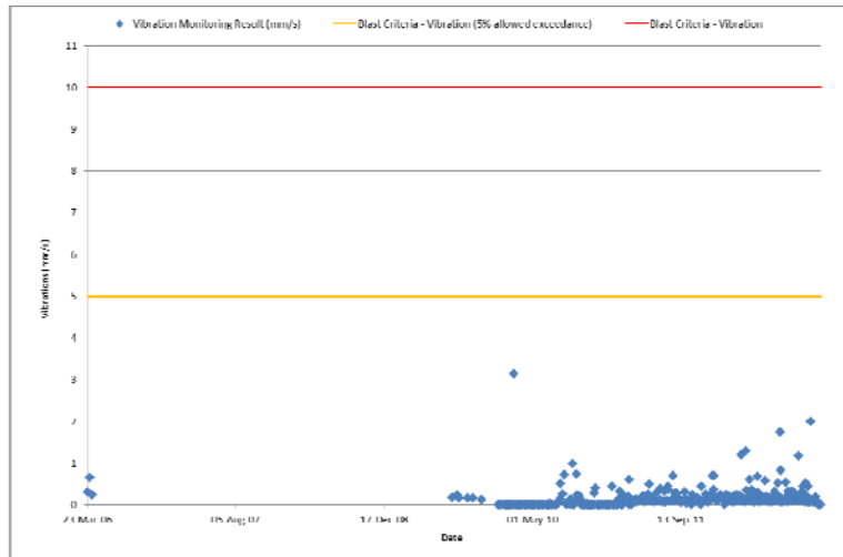
Figure 3: Historical Monitoring Results – Jim Smith’s Property (2006-2013) - Vibration
