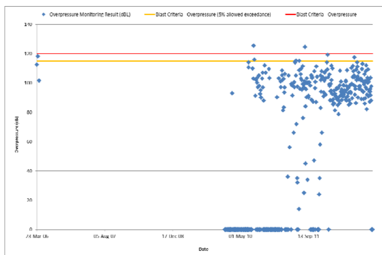
Figure 2: Historical Monitoring Results – Jim Smith’s Property (2006-2013) - Overpressure
