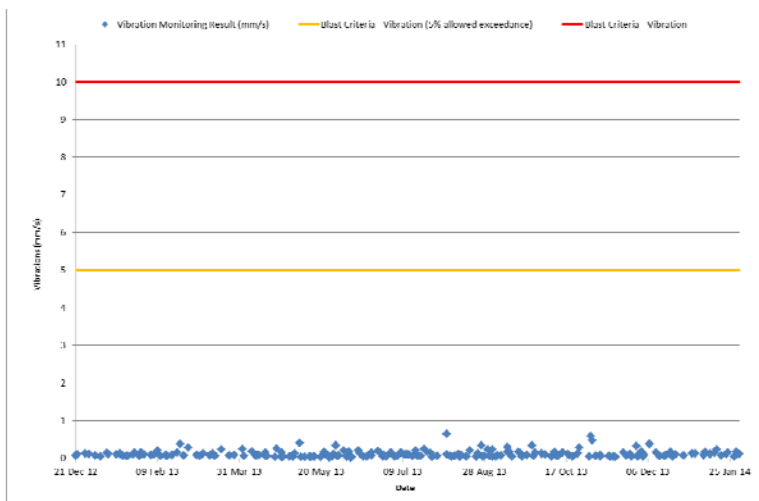
Figure 5: Historical Monitoring Results – Wollar Public School (2012-2014) – Vibration
