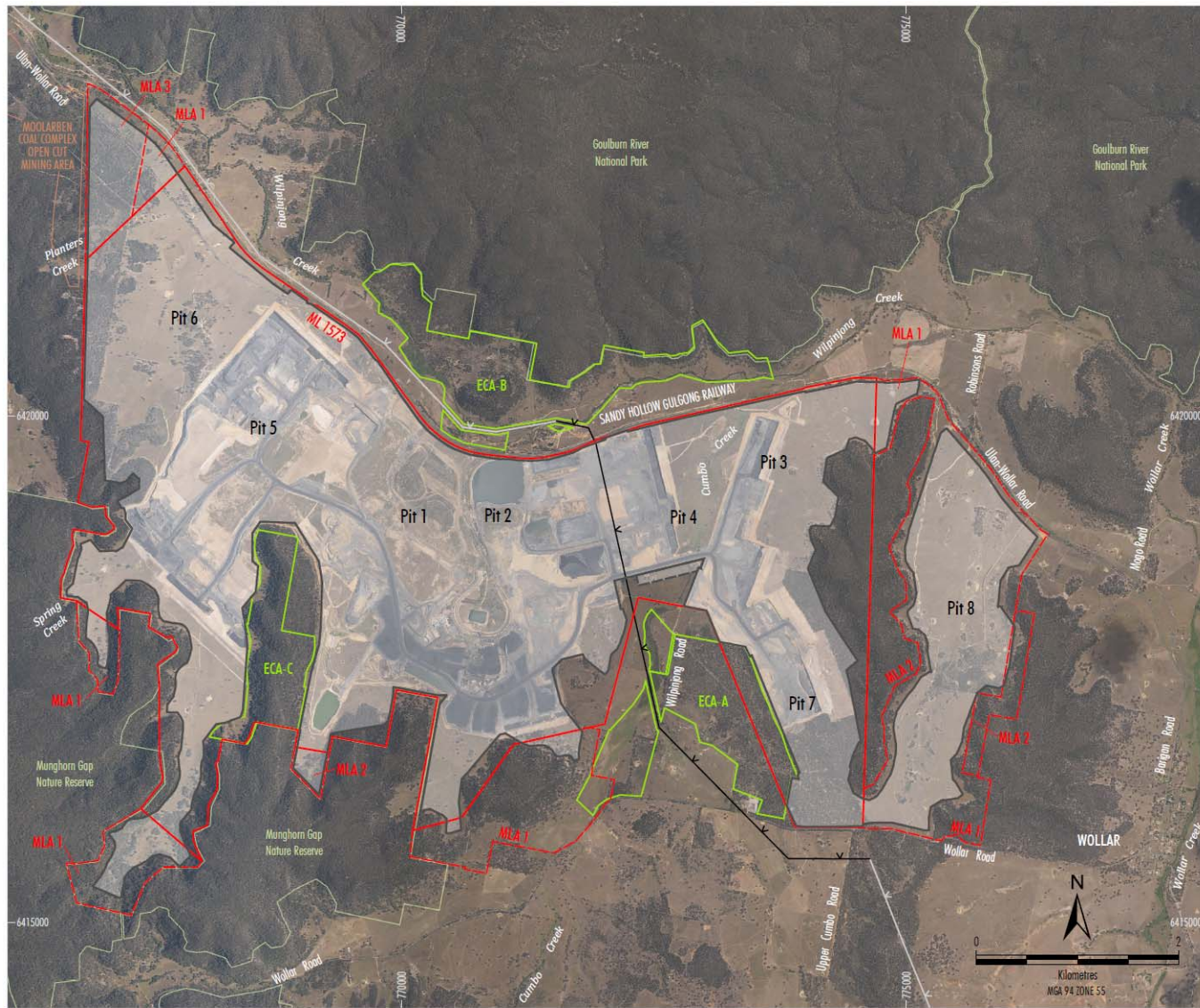
Figure 12 General Mine Layout
