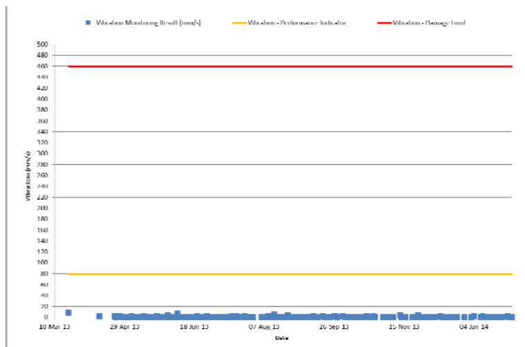
Figure 8: Historical Monitoring Results – Aboriginal Site 153 (2013-2014) – Vibration 6
